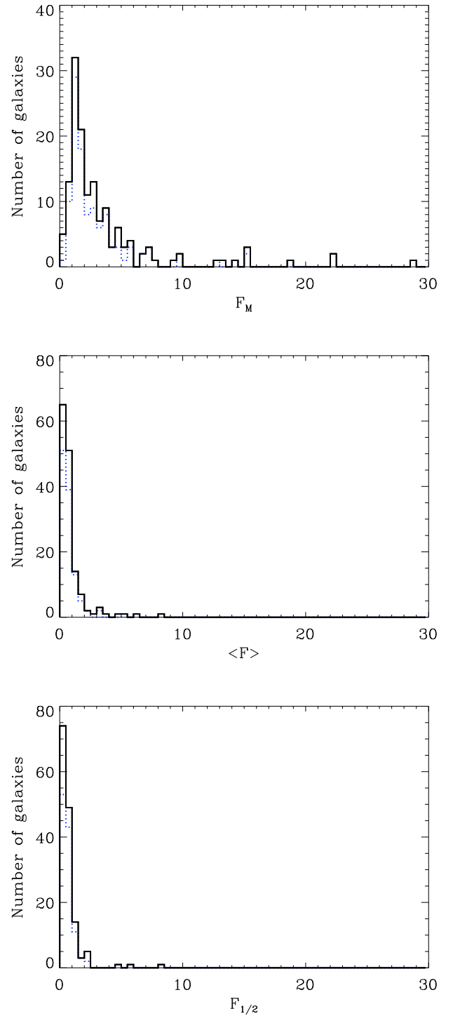
Fig. 5. The distribution of the 148 sample bulges as a function of their maximum (top panel), mean (middle panel), and median (bottom panel) intrinsic flattening, plotted with a solid line. In each panel, the dotted line refers to the distribution of the 115 sample bulges with \phi_C > \phi_M .
