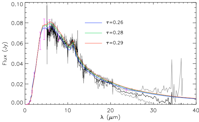
Fig. 4. The sensitivity of the 2D dust model output to optical depth. The SAGE Epoch 1 photometry for LPV 28579 is allowed a 3\sigma variation (magenta error bars), and the spectroscopy is kept to within 1\sigma (gray curves). Model SEDs for 11.3\ \mu\text{m} optical depth values spanning this range of allowed fluxes are also shown. The optical depth for good fits ranges from 0.26 (blue curve) to 0.29 (red curve). The best-fit curve for \tau = 0.28 (green) is also shown for comparison.
