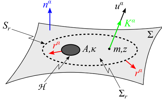
FIG. 3 (color online). A spatial slice \Sigma of a circular-orbit compact binary spacetime. The black hole is characterized by its horizon area A and uniform surface gravity \kappa , while the point particle has a mass m and redshift factor z = 1/u^t , and is such that its four-velocity reads u^\alpha = u^t K^\alpha .
