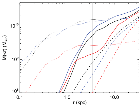
Figure 11. Integrated mass profiles at z = 6 of the cold filaments (solid), star-forming gas (dotted) and hot gas (dashed) for the nofeedback (black), noAGN (blue) and AGN case (red). The vertical grey line corresponds to 0.1 r_{\text{vir}} . Profiles in the noAGN case are very similar to the nofeedback case: only a small quantity of hot gas is removed by SNe. AGN feedback, however, expels large amounts of gas from the centre of the halo.
