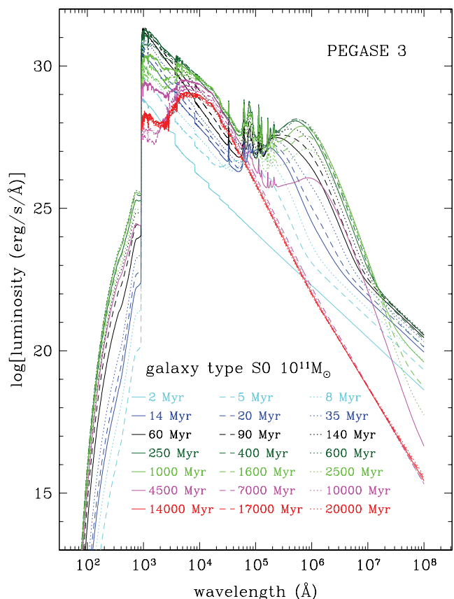
Figure 2. An example of SED templates for a 10^{11} M_{\odot} S0-type galaxy at various stages of evolution as computed with PEGASE.3. The 1- \mu\text{m} peak of giant stars appears at ages \geq 1 Gyr. Input parameters are: star formation rate = 2 \times 10^{-3} \times current gas mass per Myr; an infall time-scale of 100 Myr; galactic winds ejecting gas and dust at 5 Gyr; a Kroupa IMF; and a spheroidal extinction model (see text for details).
