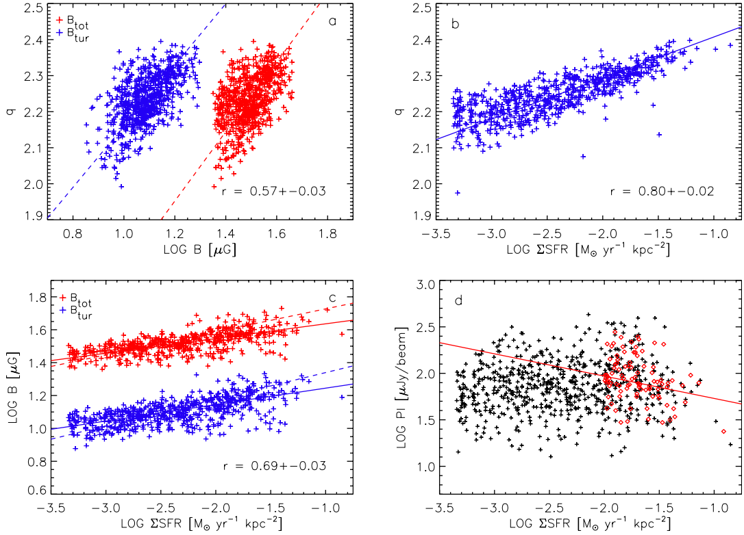
Fig. 9. Radio-IR correlation (q-parameter) versus total and turbulent magnetic field strength a) and star formation surface density \Sigma_{\text{SFR}} b) . The magnetic field strength- \Sigma_{\text{SFR}} relation is shown for the total, turbulent c) , and the ordered magnetic field strength measured by the degree of polarization d) . The lines in the upper panels are the bisector fits. The solid lines in c) and d) show the ordinary least square fit, and the dashed line the bisector fit. In panel d) , the binned data points (diamonds) are fitted for \Sigma_{\text{SFR}} \geq 0.01 M_{\odot} \text{ yr}^{-1} \text{ kpc}^{-2} (solid line). In panels a) and c) , the total magnetic field is shifted up by 0.3 units for clarity. The nucleus is not included in these analysis.
