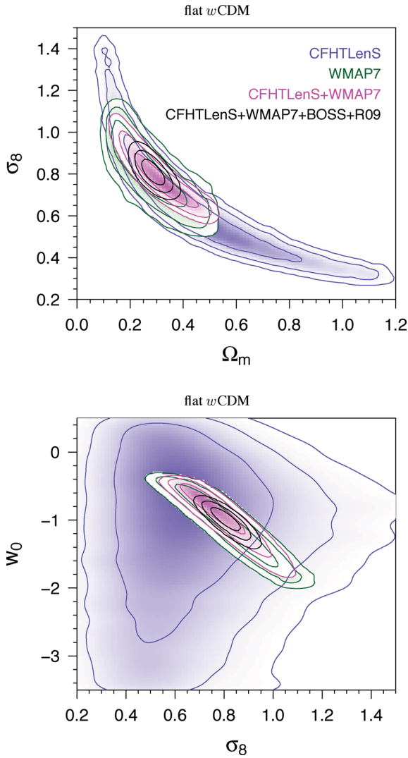
Figure 11. Marginalized posterior density contours (68.3 per cent, 95.5 per cent, 99.7 per cent) for CFHTLenS (blue contours), WMAP7 (green), CFHTLenS+ WMAP7 (magenta) and CFHTLenS+ WMAP7 +BOSS+R09 (black). The model is flat w CDM.
