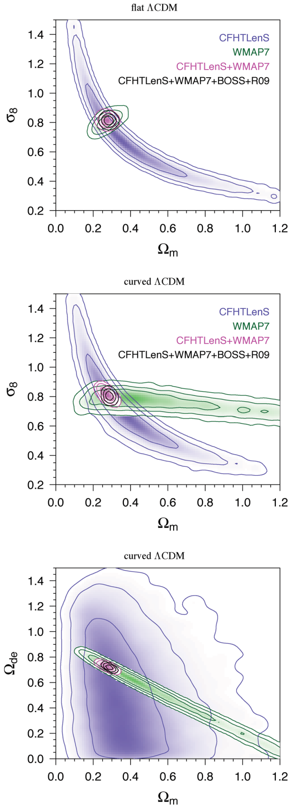
Figure 10. Marginalized posterior density contours (68.3 per cent, 95.5 per cent, 99.7 per cent) for CFHTLenS (blue contours), WMAP7 (green), CFHTLenS+ WMAP7 (red) and CFHTLenS+ WMAP7 +BOSS+R09 (black). The model is flat \Lambda CDM (left-hand panel) and curved \Lambda CDM (middle and right panels), respectively.
