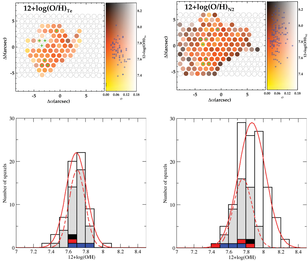
Figure 7. Top panels: maps of oxygen abundance ( 12+\log O/H ) derived from T_e[O\text{III}] (left) and the N2 parameter (right); right-hand side colour bars and green crosses are as indicated in Fig. 5. The corresponding histograms are in the bottom row. The grey bars indicate the spaxels where we measure the nebular He II \lambda 4686 , blue bars represent the spaxels showing only the blue WR bump (i.e. the spaxels within knot A; see Figs 2 and 5), red bars indicate the spaxels within knot B (see Figs 2 and 5), all showing both the blue and red WR bumps, and the black bar represents the individual spaxel in the NW with both the blue and red WR bump detection (i.e. knot C in Figs 2 and 5). The solid and dashed curves represent the Gaussian fits to all spaxels and only the spaxels where we detect nebular He II \lambda 4686 line, respectively. The uncertainties of (O/H)_{N2} are obtained by propagating the errors of [N\text{II}] and H\alpha lines (involved in the N2 parameter) in the derivation of O/H , and do not consider the typical uncertainty associated with the N2 parameter ( \sim 0.3 dex).
