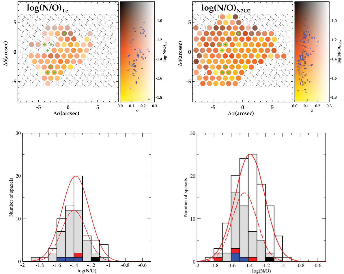
Figure 8. Top panels: maps of \log(N/O) derived from T_e[O\text{ III}] (left) and the N2O2 parameter (right); right-hand side colour bars and green crosses are as indicated in Fig. 5. The corresponding histograms are in the bottom row; the colouring of the bars and curves are the same as in Fig. 7. The uncertainties of (N/O)_{N2O2} are obtained by propagating the errors of [N\text{ II}] and [O\text{ II}] lines (involved in the N2O2 parameter) in the derivation of N/O , and do not consider the typical uncertainty associated with the N2O2 parameter ( \sim 0.25 dex).
