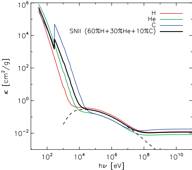
Figure 8. Atomic scattering opacities of high-energy photons on H, He, C and a mixture of composition mimicking that of a Type II core-collapse SN ejecta (60 per cent H, 30 per cent He and 10 per cent C). The black dashed line indicates the contribution of Compton scattering in the latter composition case. From http://henke.lbl.gov/optical_constants/ for 30 \text{ eV} \leq h\nu < 1 \text{ keV} and http://physics.nist.gov/cgi-bin/Xcom/ for 1 \text{ keV} \leq h\nu < 100 \text{ GeV} .
