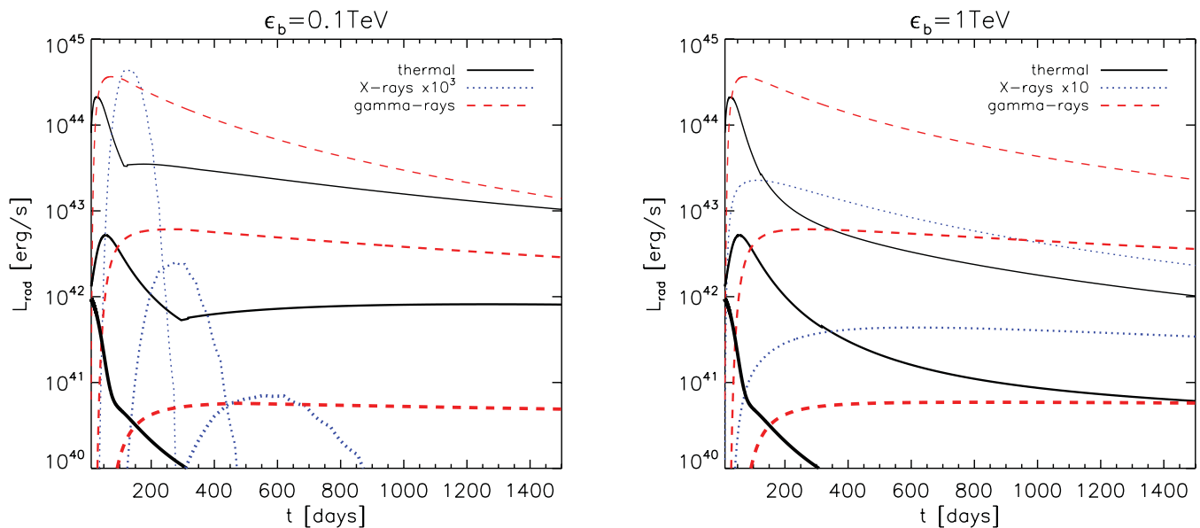
Figure 9. Thermal emission (black solid lines), non-thermal X-ray emission (blue dotted line) at energy indicated in Fig. 7 (emitted mostly between 0.1 and 100 keV for \epsilon_b = 0.1 TeV, and between around 100 keV and 1 GeV for \epsilon_b = 1 TeV), and non-thermal gamma-ray emission (red dashed line) at 0.1 TeV (left-hand panel) and 1 TeV (right-hand panel), expected from an SN ejecta with M_{ej} = 5 M_{\odot} and E_{ej} = 10^{51} erg s^{-1} , embedding a pulsar with a dipole magnetic field of B = 10^{13} G and period P_i = 1, 3, 10 ms (increasing thickness), assuming \eta_B = 0.01 , \eta_e = 1 - \eta_B and a break energy \epsilon_b = 0.1 TeV (left-hand panel) and \epsilon_b = 1 TeV (right-hand panel). Caution: for visibility, the X-ray luminosity is multiplied by 10^3 in the left-hand panel and by 10 in the right-hand panel. The slight discontinuities are numerical artefacts.
