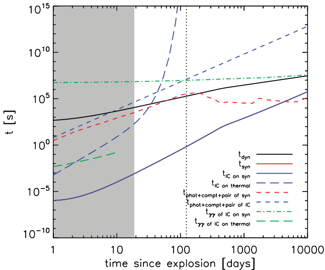
Figure 6. Time-scales at play in the radiation emission of a PWN, for the same system as in Fig. 4, assuming an electron injection break energy \epsilon_b = 0.1 TeV, and \eta_B = 0.01 . The dynamical time-scale, t_{\text{dyn}} (black solid line), and cooling time-scales via synchrotron, t_{\text{syn}} (red solid line), via self-Compton, t_{\text{IC,syn}} (blue solid line) and via IC off thermal photons (blue long-dashed line) are compared to thermalization time-scales. The thermalization time-scales via photoelectric absorption, Compton scattering and pair production are shown in the dashed lines (in red for the synchrotron photons and blue for the IC photons). Absorption by \gamma\text{--}\gamma interaction at high energies is shown in the green lines (dot-dashed for the interaction between IC photons on synchrotron photons, and long-dashed for the interaction of IC photons on the thermal photons of the SN ejecta). The grey shaded region corresponds to t < t_d , where the Arnett (1980) approximation is not valid, and the dotted line indicates t = t_{\text{thin}} .
