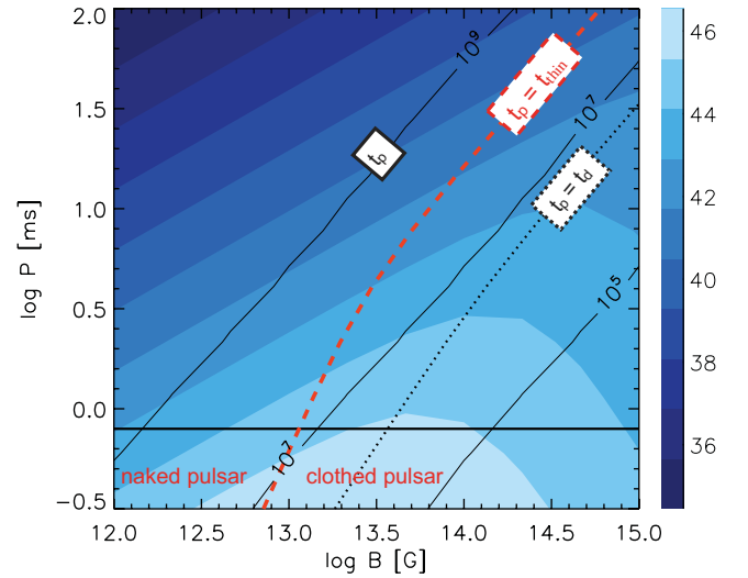
Figure 1. Contour plot of the bolometric luminosity of SN+PWN systems at 1 yr after the explosion (the fraction of wind energy converted into radiation, as defined in Section 3, is set to \eta_\gamma = 1 ), as a function of the initial period P and magnetic field B . The various regimes for radiative emissions described in Section 2.1 are represented. The solid lines indicate the pulsar spin-down time-scale in seconds (equation 5). The red dashed lines represent the pulsar population for which t_p = t_{\text{thin}} , and separate naked and clothed pulsars (see text). The dotted lines represent t_p = t_{\text{d}} .
