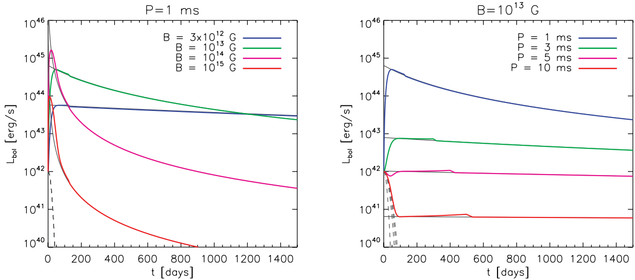
Figure 5. Evolution of the bolometric radiated luminosity of the SN as a function of time. The pulsar has a dipole magnetic field of increasing strength as indicated, and a period P_i = 1 ms (left-hand panel), and B = 10^{13} G and increasing periods as indicated in the legend (right-hand panel). The SN ejecta has M_{ej} = 5 M_{\odot} and E_{ej} = 10^{51} erg. The grey lines give the evolution of the pulsar luminosity L_p for each initial spin period. The grey dashed lines are the contribution of the ordinary core-collapse SN to the radiated luminosity L_{SN} . We have assumed \eta_{\gamma} = 1 . The slight discontinuity is due to the numerical calculation of the integral in equation (20), and marks the transition between t < t_{thin} and t > t_{thin} .
