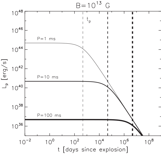
Figure 3. Evolution of the pulsar luminosity L_p as a function of time, for magnetic dipole spin-down. The pulsar has a dipole magnetic field of B = 10^{13} G, and a period P_i = 1, 10, 100 ms (increasing thickness). The vertical dashed lines correspond to the spin-down time-scale t_p for each initial spin period.
