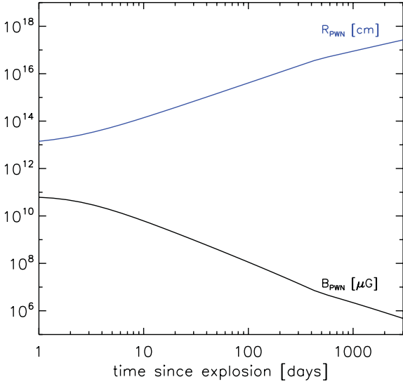
Figure 4. Evolution in time of the radius, R_{\text{PWN}} , and the magnetic field strength, B_{\text{PWN}} , of a PWN, assuming no shell disruption (equations 10 and 12) and \eta_B = 0.01 , calculated for an SN ejecta with M_{\text{ej}} = 5 M_{\odot} and E_{\text{ej}} = 10^{51} erg \text{s}^{-1} , embedding a pulsar with a dipole magnetic field of B = 10^{13} G and period P_1 = 1 ms.
