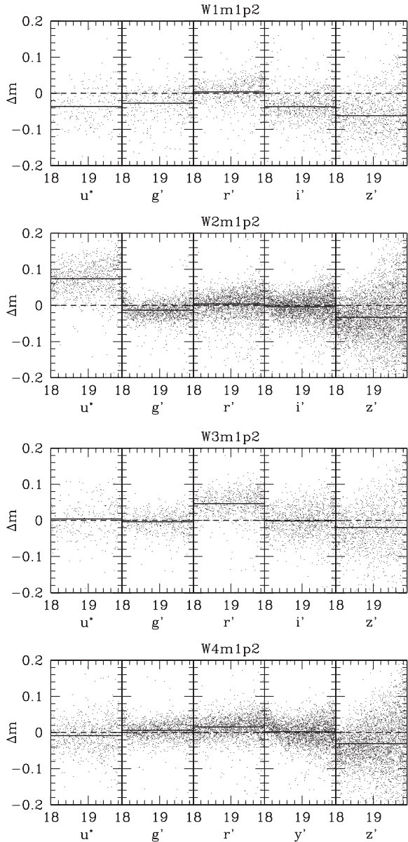
Figure 10. Magnitude comparisons between SDSS stars with and CFHTLenS sources for the fields W1m1p2 with x \in \{1, 2, 3, 4\} . The solid horizontal lines indicate \langle \Delta m \rangle . The precise values of the mean offsets and formal standard deviations can be found in Table A1. Note that W4 and W2 are at significantly lower galactic latitude than W1 and W3; thus, the stellar density in the latter two is substantially lower.
