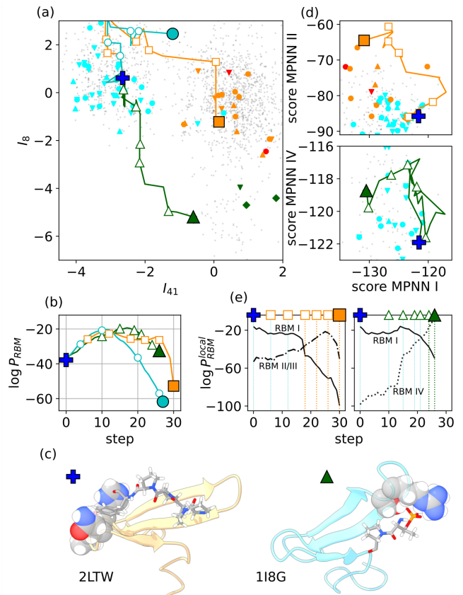
FIG. 2. Mutational paths of the WW domain using RBM trained on the PFAM PF00397 family, see Supplemental Material, Sec. 3 for details about implementation. (a) Natural sequences \mathbf{v} (grey dots) projected onto the plane of inputs I_\mu (here M = 50 ) of two hidden units clustering sequences according to the types of ligands they bind [24]: I (cyan), II (red), III (orange), IV (green). Marked sequences: Upper (Lower) triangles: natural (artificial), from [29]. Diamond: natural, from [30]. Blue cross represents the YAP1 domain. Lines show the projection of three representative paths connecting YAP1 to sequences in classes I (circle), II (square) and IV (triangle). Intermediate sequences (empty symbols) are listed in Supplemental Material, Sec. 5.1. Parameters: \beta = 3 , \Lambda = 0.1 . (b) \log P_{RBM} for sequences along the paths. (c) Complexes (WW domain and cognate peptides) for classes I (blue cross) and IV (green triangle) [31]. Atoms corresponding to the two binding pockets are highlighted. (d) Normalized ProteinMPNN scores for binding affinity, see Supplemental Material, Sec. 5.4. x -axis measures the affinity to class I reference structure while y -axes show affinity to classes II/III (Top) and IV (Bottom) reference structure respectively. (e) Log-likelihood along the paths from I to II (Left) and from I to IV (Right) according to class-specific RBM trained on sequences in the three quadrants (Solid: I, Dot-dashed: II/III, Dotted: IV).
