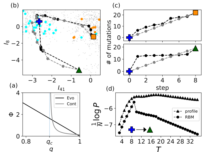
FIG. 3. Mean-field theory of mutational paths for the RBM model trained on WW domain. (a) Sketches of the potentials \Phi_{\text{Evo}} (black) and \Phi_{\text{Cont}} (gray) vs. q . (b) Same two-dimensional representation as in Fig. 2(a) for the mean-field paths with Evo (black lines) and Cont (gray lines) potentials. (c) Cumulative numbers of mutations vs. t . Here, \mu = 10^{-5} and \gamma = 0.9 , so that the cumulative numbers match for t = T . (d) Log-probability of joining class I and class IV natural WW domains in T steps with the profile (triangles) and RBM (circles) models. Jumps signal the onset of several new mutations, e.g. 4 in the mean-field free path at T = 10 .
