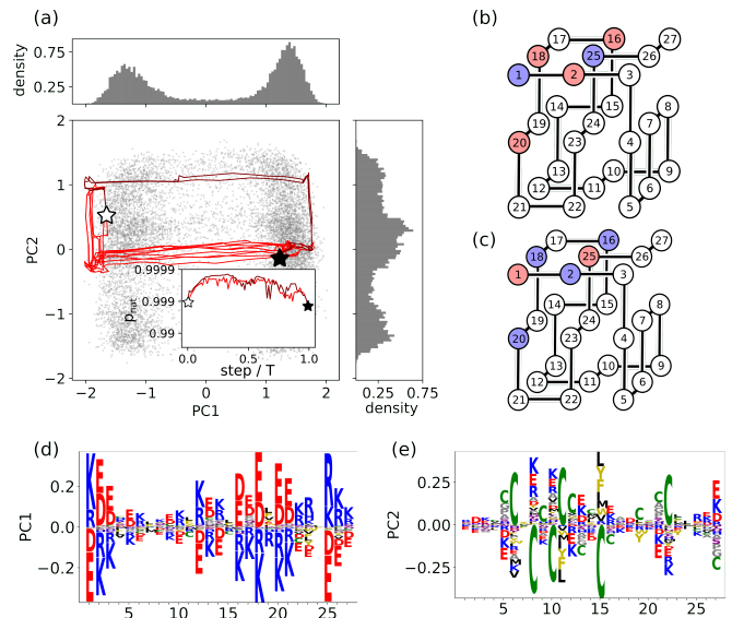
FIG. 1. Mutational paths for lattice proteins , joining sequences \star = \text{DRGIQCLAQMFEKEMRKKRRKCYLECD} and \blackstar = \text{RECCAVCHQRFKDKIDEDYEDAWLKC} N belonging to the family with structure shown in b) and c). Red and blue colors respectively correspond to negatively and positively charged amino acids. Cysteine is denoted by a green C. (a) Projections of 10^4 LP sequences in the family (grey dots) along the top two PC of their correlation matrix. Red and maroon lines show some representative paths sampled from Eq. (2). The relative numbers of maroon (2) and red (10) paths respect the statistics over all sampled paths. Parameter values: \beta = 3 , \Lambda = 2 , T = 82 . Sides: histograms of projections along PC1 (top) and PC2 (right). Inset: folding probability p_{nat} along each path vs. number of mutations/ T . (b,c) The fold of the LP family is stabilized by alternating configurations of charges. (d,e) Sequence logos of PC1 and PC2.
