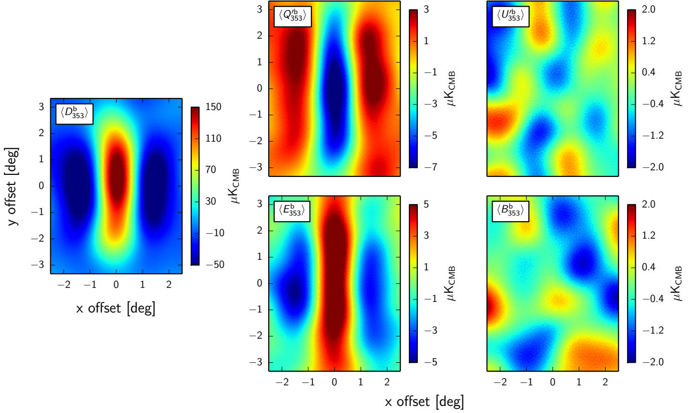
Fig. 10. Mean images of the Planck \langle D_{353}^b \rangle , \langle Q_{353}^b \rangle , \langle U_{353}^b \rangle , \langle E_{353}^b \rangle , and \langle B_{353}^b \rangle maps over the \lambda_- filaments.
