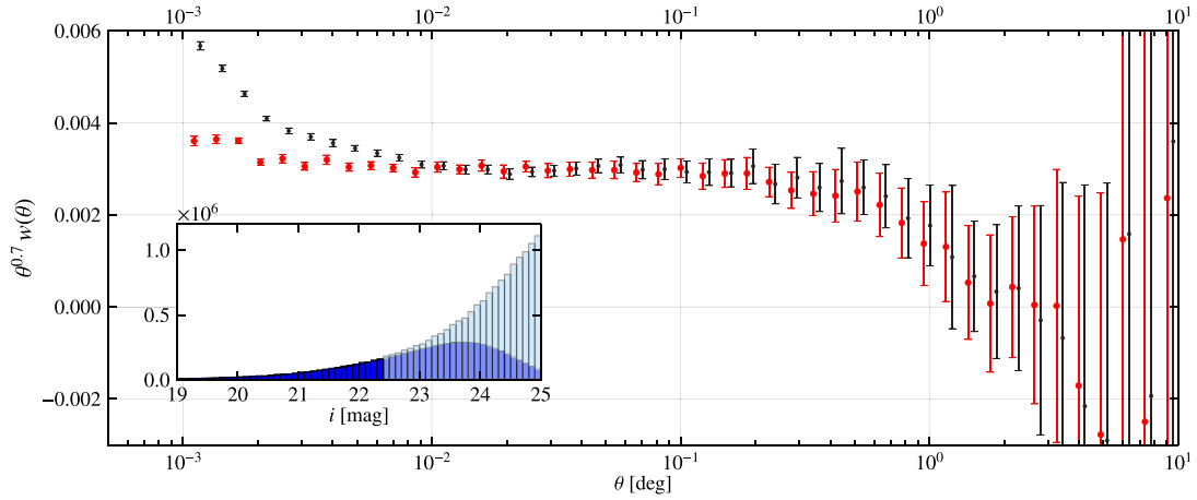
Figure C1. Angular clustering measurements using a sample similar to that of Crocce et al. (2016), with BALROG (red points) and uniform randoms (black points). The figure is similar to Fig. 13. Selection cuts are discussed in Section 3.4 and Appendix A. Shown in the inset, a magnitude cut of 18 < \text{MAG\_AUTO\_I} < 22.5 has been applied; blue is the observed magnitude distribution and light blue is the truth magnitude distribution from BALROG. The correlation functions have been scaled by the approximate power-law slope. The results suggest that the measurements made in Crocce et al. (2016) are unaffected by significant sources of systematic bias at scales \theta > 0.01 .
