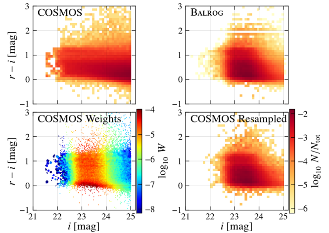
Figure 10. COSMOS sample selection. The heat map coloured histograms plot normalized counts. Top left: i -band magnitudes and r - i colours for the full COSMOS catalogue after basic quality cuts. Top right: distribution of i -band magnitude and r - i colours using truth catalogue properties of BALROG galaxies in our faint sample. Bottom left: (unnormalized) weights applied in the i, r - i colour plane to COSMOS galaxies in order to match the DES truth distribution. Bottom right: i -band magnitudes, r - i colours of the reweighted COSMOS sample.
