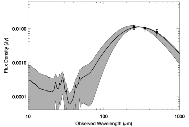
Figure 4. An example fit of a starburst model to the SPIRE fluxes extracted from the stacked data (Section 3.3). This fit is for the seventh M_i bin (see supplementary online materials). The black line shows the best-fitting SED, while the shaded region shows the range in SED shapes that are consistent with the range in starburst luminosity for this fit.
