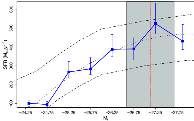
Figure 6. Star formation rate as a function of M_i (Section 4.2). The blue points show the data and the black lines show the model in equation (2) and its 90 per cent confidence interval. The vertical red line and grey shaded region show the M_i and uncertainty for L^* quasars at 2.5 < z < 3.8 (Delvecchio et al. 2014, with K -correction to z = 2 from Richards et al. (2006b).
