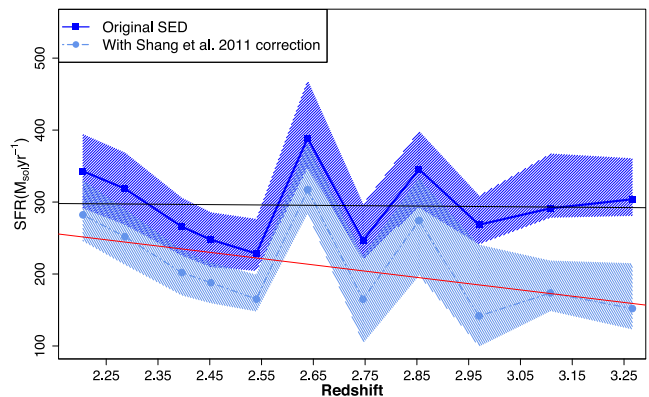
Figure 13. The effect of using the composite observed quasar SED of Shang et al. (2011) to correct the M_s - z relation in Fig. 5. The dark blue region shows the original relation while the light blue region shows the relation after normalizing the Shang et al. 2011 SED to the median M_i of that bin, extracting predicted SPIRE fluxes, and removing them before fitting. As discussed in Section 5.3 this is an overcorrection, so the light blue region should be regarded as a lower limit. Fitting a linear model to the light blue points gives a slight negative slope, but consistent to within 2\sigma with a flat relation.
