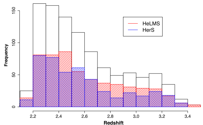
Figure 3. Redshift distributions for the quasars in HeLMS and HerS (red and blue hatched histograms, respectively) and for all SDSS DR9 quasars in Stripe 82 with uniform flag >0 and 2.15 < z < 3.5 (white solid).
