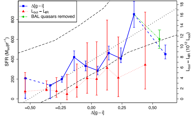
Figure 7. Star formation rate versus \Delta[g - i] (Section 4.3). The blue points show the data. The solid blue line shows the range in \Delta[g - i] over which we have enough objects to be confident of the results (Section 3.1). The black lines show the model in equation (3) and its 90 per cent confidence interval (Section 4.2). The points connected by dashed blue lines are those for which we have only a few objects, and are thus less trustworthy. The green point is the same as the last blue point but with the BAL quasars removed. The red line shows the difference between the bolometric and infrared luminosities as a function of \Delta[g - i] , according to the right-hand scale (Section 6.2).
