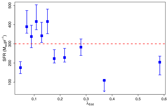
Figure 18. Star formation rate as a function of \lambda_{\text{edd}} (equation 17). The red horizontal line is the mean star formation rate derived from the model fit in Fig. 5.
