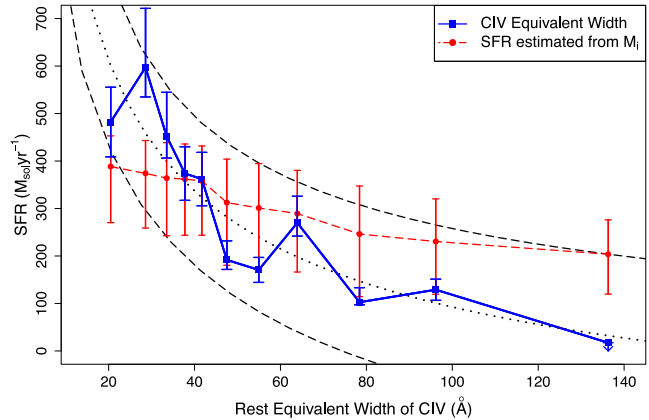
Figure 9. Star formation rate versus CIV EW (Section 4.4). The blue points show the data, while the black lines show the model in equation (8) and the 90 per cent confidence interval. The red line is the result of using equation (2) to calculate the predicted star formation rate associated with the mean M_i for each bin.
