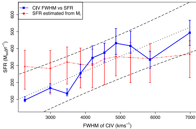
Figure 8. Star formation rate versus CIV FWHM (Section 4.4). The blue points show the data, while the black lines show the model in equation (6) and the 90 per cent confidence interval. The red line is the result of using equation (2) to calculate the predicted star formation rate associated with the mean M_i for each bin.
