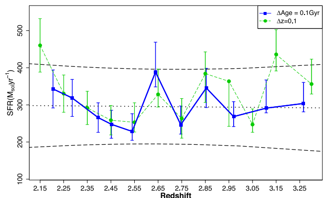
Figure 5. The evolution with redshift of star formation rates in quasar hosts (Section 4.1). The data are shown for bins of equal width in both age (blue) and redshift (green). The black lines show the model fit in equation (1) and the 90 per cent confidence interval.
