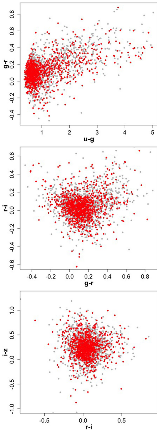
Figure 2. Observed-frame colour–colour diagrams for our sample (red) and all SDSS DR9 quasars in Stripe 82 with uniform flag >0 and 2.15 < z < 3.5 (grey). The distributions are identical by visual inspection, and indistinguishable via a K–S test.
