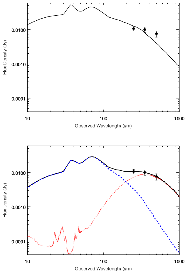
Figure 12. Examples of including AGN models when fitting to the SPIRE data. The top panel shows the best-fitting pure AGN model to the same SPIRE flux densities as in Fig. 4. The model can reproduce the 250 \mu\text{m} and 350 \mu\text{m} data but misses the 500 \mu\text{m} data. The lower panel shows the result of simultaneously fitting both AGN (blue) and starburst (red) models to the data. The fit is under constrained but still predicts that the starburst contributes most of the SPIRE emission.
