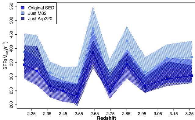
Figure 11. The effect of SED library choice on the \dot{M}_s - z relation. This plot reproduces the \Delta t binned data in Fig. 5 (medium blue), and adds the same relation derived using more restricted SED libraries; ones that closely resemble M82 (light blue) and Arp220 (dark blue).
