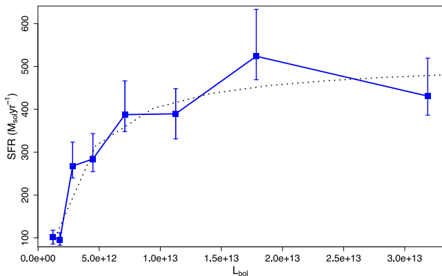
Figure 15. Star formation rate as a function of bolometric accretion luminosity. The L_b values were computed via equation (10). The dotted line is the relation in equation (11).
