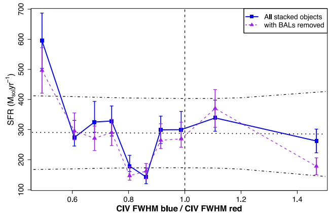
Figure 10. Star formation rate versus CIV asymmetry, measured via the blue over red side E_C (Section 4.4). The blue points show the data, while the black lines show the model in equation (9) and the 90 per cent confidence intervals. The purple line reproduces the blue line, but with the BAL quasars removed.
