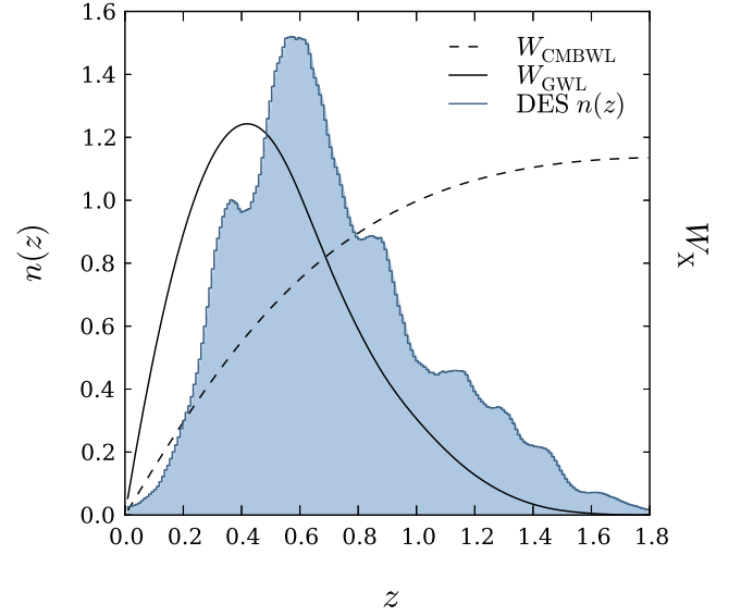
Figure 1. The blue region shows the redshift distribution of the source galaxies from DES over our chosen redshift range, 0.3 < z < 1.3 , normalized such that the total area under the curve equals unity. The solid and dashed black lines show the lensing kernels for GWL and CMBWL respectively. Each weight function has been normalized for visual comparison with the n(z) . The DES sources are taken from the ngmix shape catalogue and we use the SkyNet2 photo- z estimates (see Sections 3.1.1 and 3.1.2 for more details).
