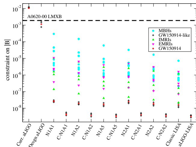
FIG. 1. 1\sigma constraints on the BH dipole flux parameter B from various sources—GW150914-like BH binaries (stars and pluses), massive BH binaries (filled circles), and EMRIs/IMRIs (filled triangles)—as a function of the instrument—aLIGO at the time of the GW150914 event (Curr. aLIGO), aLIGO at design sensitivity (Design aLIGO), various six-link eLISA configurations ( N \times A \times ) with target/pessimistic low-frequency noise ( N2/N1 ) and 1 Gm/2 Gm arms ( A1/A2 ), a Classic LISA design with six links, 5-Gm arms and target-level low-frequency noise, and joint observations by design aLIGO and eLISA ( C-N \times A \times ), or by design aLIGO and Classic LISA (aLIGO-LISA). For comparison, we also include the current constraint on vacuum dipole radiation from LMXB A0620-00 [65]. The combined aLIGO-eLISA observation of GW150914-like sources leads to the most stringent constraints, which are 6 orders of magnitude stronger than current bounds.
