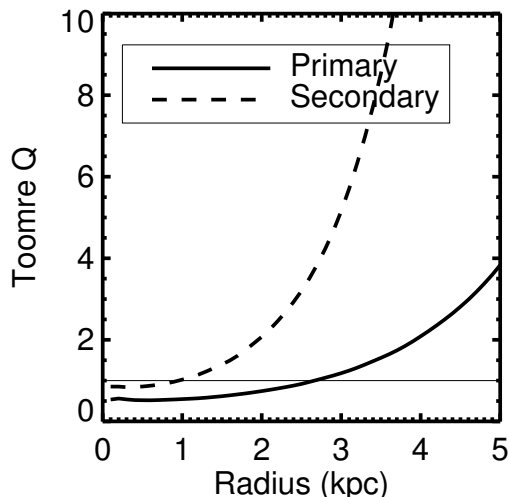
Fig. 7. Toomre Q parameter estimated as a function of radius for the initial disk galaxies in a 4:1 merger in RAMSES. A horizontal line marks the marginally stable value Q = 1 . At a gas temperature of 10^3 K (which is effectively enforced by the Jeans polytrope temperature minimum), the secondary galaxy is substantially more stable than the primary, and it remains stable or near marginal stability at all radii. This leads to a low SFR in the secondary. In the GASOLINE simulations without a Jeans polytrope, the secondary has higher SFRs.
