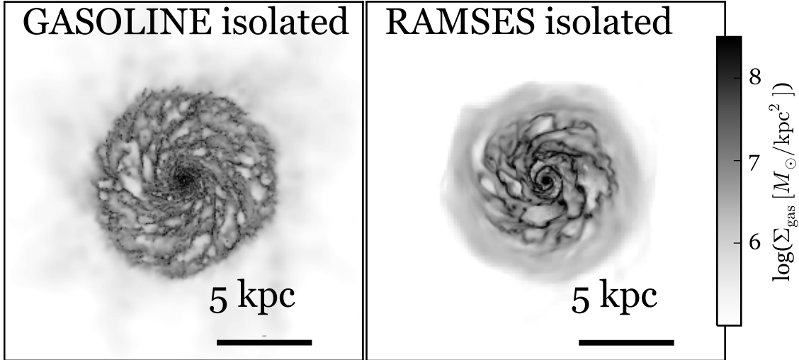
Fig. 3. Face-on images of gas surface density of an isolated disk galaxy simulation using GASOLINE ( left ) and RAMSES ( right ). The characteristic sizes of gas structures are larger in RAMSES than in GASOLINE due partly to the Jeans polytrope pressure floor implemented in RAMSES and partly to differences in more fundamental aspects of the codes (e.g., hydrodynamic or gravity solvers).
