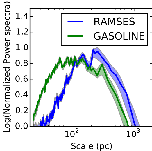
Fig. 4. Power spectra of gas surface density fluctuations in isolated GASOLINE and RAMSES galaxies. The power spectra are normalized by a third-degree power law to highlight the differences between simulations. Shaded error regions indicate the 10–90th percentile range from bootstrap resampling. GASOLINE shows more power at small scales and less power at large scales, emphasizing that gas structures in our GASOLINE simulations tend to have smaller sizes than those in RAMSES.
