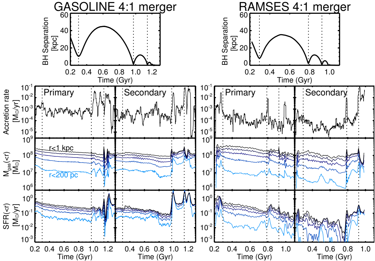
Fig. 2. BH separation in kpc ( top ), black hole accretion rate (BHAR) in M_{\odot} \text{ yr}^{-1} ( second row ), gas mass in M_{\odot} within spheres up to 1 kpc in radius ( third row ), and SFR in M_{\odot} \text{ yr}^{-1} within the same spheres ( bottom row ) vs. time for a 4:1 merger with GASOLINE ( left ) and RAMSES ( right ). For each simulation, we show quantities for the primary galaxy/BH on the left, and the secondary galaxy/BH on the right. We show gas masses and SFRs within radii of 200 pc to 1 kpc, in increments of 200 pc. Quantities are smoothed on 10 Myr timescales. Note that time-axes differ by \sim 20\% (see Sect. 3.2.1). Vertical dotted lines mark local minima in the separation between the two black holes in all panels. The GASOLINE and RAMSES simulations show qualitatively similar results: enhanced accretion and star formation rates at the second pericenter, and especially at the third pericenter/coalescence.
