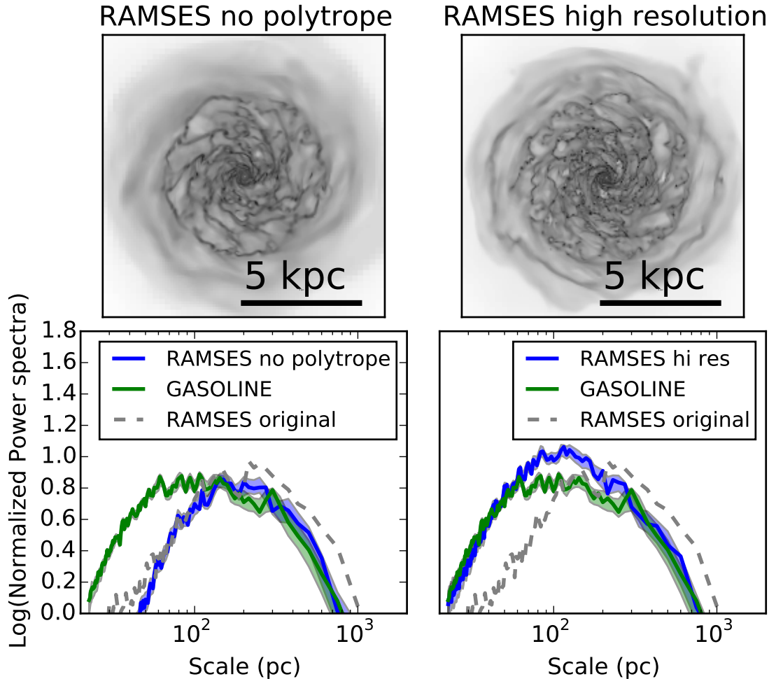
Fig. 6. Gas surface density maps ( top ) and power spectra ( bottom ) for RAMSES simulations of isolated galaxies with different settings: Left : simulation with no Jeans polytrope pressure floor. Right : simulation with a more easily triggered refinement criterion that enables \approx 15 pc resolution throughout the galactic disk (and without the Jeans polytrope). Removing the Jeans polytrope ensures that the power on scales \geq 200 pc is similar in RAMSES and GASOLINE simulations. Enhancing the typical cell size in RAMSES leads to improved agreement between RAMSES and GASOLINE power spectra on scales \leq 50 pc at the expense of a discrepancy at moderate scales of \approx 50 – 200 pc (as well as additional computational cost).
