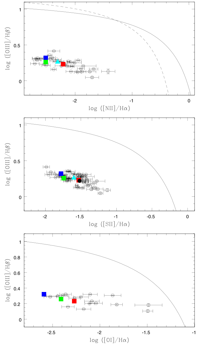
Figure 5. BPT diagnostic diagrams for IZw18. From top to bottom: \log([O\text{ III}]\lambda 5007/H\beta) versus \log([N\text{ II}]\lambda 6584/H\alpha) , \log([O\text{ III}]\lambda 5007/H\beta) versus \log([S\text{ II}]\lambda 6731,6717/H\alpha) and \log([O\text{ III}]\lambda 5007/H\beta) versus \log([O\text{ I}]\lambda 6300/H\alpha) . The symbols are as described in Fig. 4. Overplotted as a black solid curve (in all three panels) is the theoretical maximum starburst model from Kewley et al. (2001), devised to isolate objects whose emission line ratios can be accounted for by the photoionization by massive stars (below and to the left of the curve) from those where some other source of ionization is required. The black-dashed curve in the [N\text{ II}]\lambda 6584/H\alpha diagram represents the demarcation between SF galaxies (below and to the left of the curve) and AGNs defined by Kauffmann et al. (2003).
