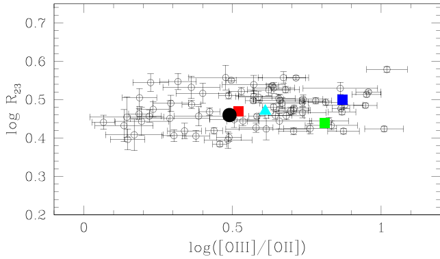
Figure 4. The relation between \log R_{23} and \log([O\text{ III}]/[O\text{ II}]) . Open circles correspond to individual spaxels from the data cube. Overplotted as blue, red, and green squares are the line ratios measured from the 1D spectra of the NW knot, SE knot and ‘plume’, respectively; the cyan triangle shows the line ratio values from the total integrated spectrum of IZw18; the black circle corresponds to the line ratios from the spectrum of the ‘halo’ of IZw18 (see Section 7 and Table 3 for details on the 1D spectra extracted for selected galaxy regions).
