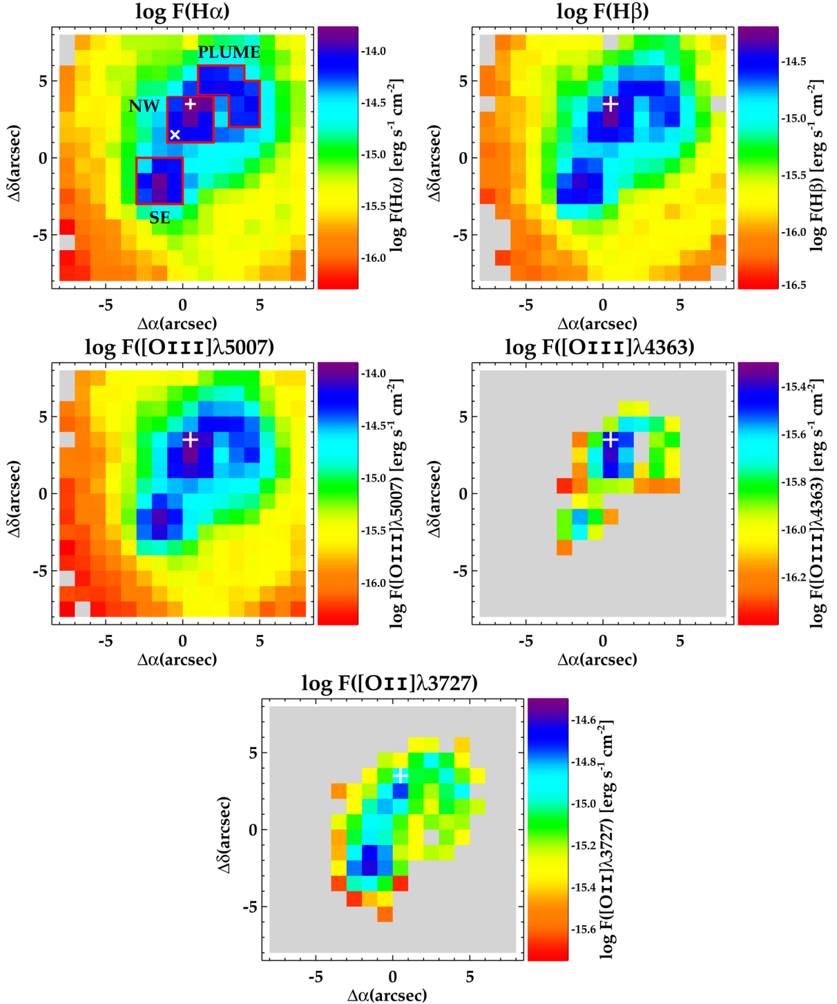
Figure 2. Emission line flux maps of IZw18: [O II] \lambda 3727 , H\beta , [O III] \lambda 4363 , [O III] \lambda 5007 , H\alpha . The spaxels with no measurements available are left grey. All maps are presented in logarithmic scale. As a guide to the reader, the peak of H\alpha emission is marked with a plus (+) sign on all maps. The cross on the H\alpha map marks the spaxel where we detect the WR feature (see Section 4). The H\alpha map also shows the boundaries of the areas that we use to create the integrated spectra of the NW and SE knots, and of the ‘plume’ region (see text for details). North is up and east to the left.
