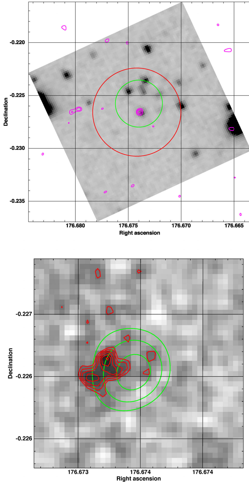
Figure 5. Top: identification of LABOCA_2 with an IRAC source. The grey-scale image is a segment of the larger IRAC 3.6 \mu\text{m} image. The magenta contours are from the SMA, at levels of 2\sigma , 3\sigma and 4\sigma , the red circle is the LABOCA beam at the position of the source, and the green circle is the SCUBA2 beam at the position of the matching source. The correct IRAC identification for this source is clear once the SMA contours are considered. Bottom: SMA contours for the LABOCA_2 source (green) overlaid on a K' band image of the source obtained from ISAAC (grey-scale and red contours). The image is 6 \times 6 arcsec in size with 0.15 arcsec pixels. The original image has been smoothed with a Gaussian of width two pixels to enhance the S/N. Note that the K' band counterpart to the SMA source is extended and seems to have a bimodal morphology, suggestive of a galaxy interaction or merger. For both images coordinates are given in degrees J2000.
