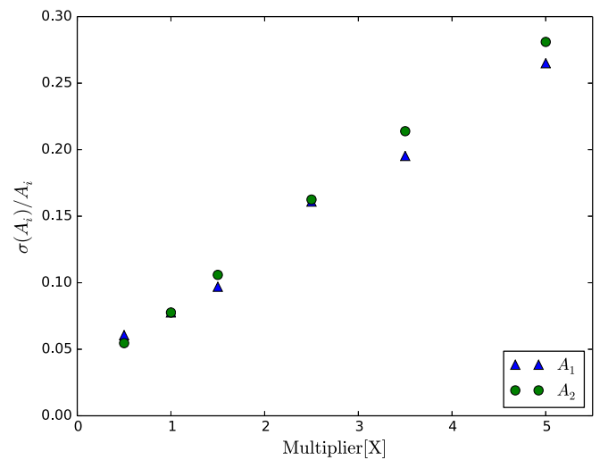
FIG. 7. Fractional 1\sigma uncertainty on A_i for different Y1 analyses, plotted against HOD prior widths as a factor of the default conservative widths.
