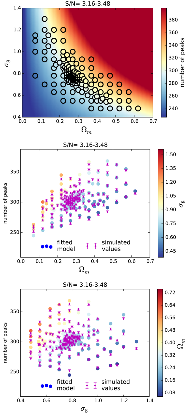
Figure B1. Modelling the number of peaks as a function of cosmology. The top panel shows the peak count for one S/N bin (3.16–3.48), as a function of the \Omega_m – \sigma_8 parameters. The grid of simulations is shown with open circles. The colour shows the interpolated peak count. Middle and bottom panels show the peak count as a function of a single cosmological parameter ( \Omega_m and \sigma_8 for middle and bottom panels respectively), with the other marked in the colour scale. The magenta points mark the number of peaks calculated from simulations, with error bars representing the uncertainty on the mean from many noise realizations.
