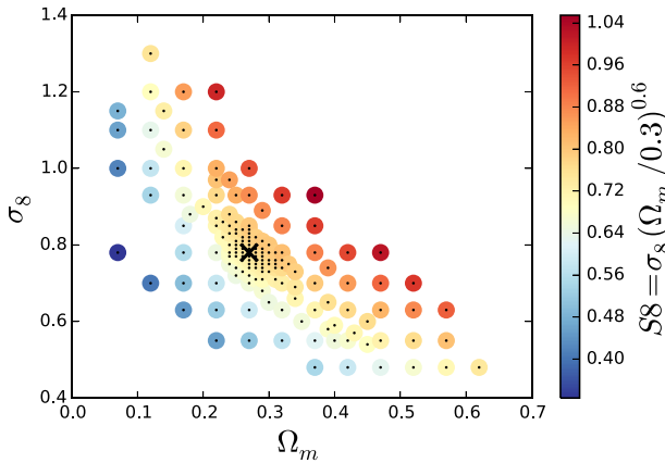
Figure 1. The grid of cosmological models in the simulations from Dietrich & Hartlap (2010). Colour corresponds to the value of S_8 = \sigma_8(\Omega_m/0.3)^{0.6} parameter. The central cosmological model is marked by a black cross. Other cosmological parameters for these simulations were: h_{70} = 1 , n_s = 1 and \Omega_b = 0.04 .
