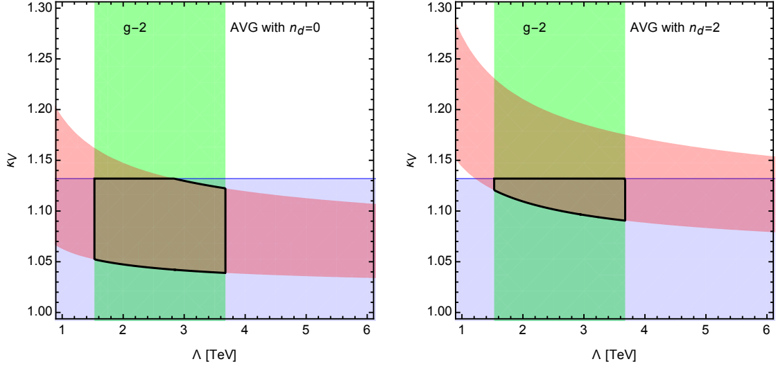
Figure 2: Allowed regions at 99% Confidence Level ( 3\sigma ) from electroweak precision (red) and the direct \kappa_V measurement (blue). The green vertical band corresponds to the region preferred by the muon g-2 anomaly. The two panels correspond to vanishing UV contribution to S (left) and n_d = 2 (right). The regions compatible with all bounds are highlighted by the black contour.
