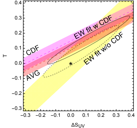
Figure 1: Comparison of the new CDF measurement of the W mass (magenta band) to the precision measurements, represented by the ellipses with (solid) and without (dashed) the CDF result. The yellow band indicates the bound stemming from asymmetries and direct s_W^2 determination. The red band represents our naive average that includes the CDF result. All bounds are shown at 95% confidence level (i.e. 2\sigma ).
