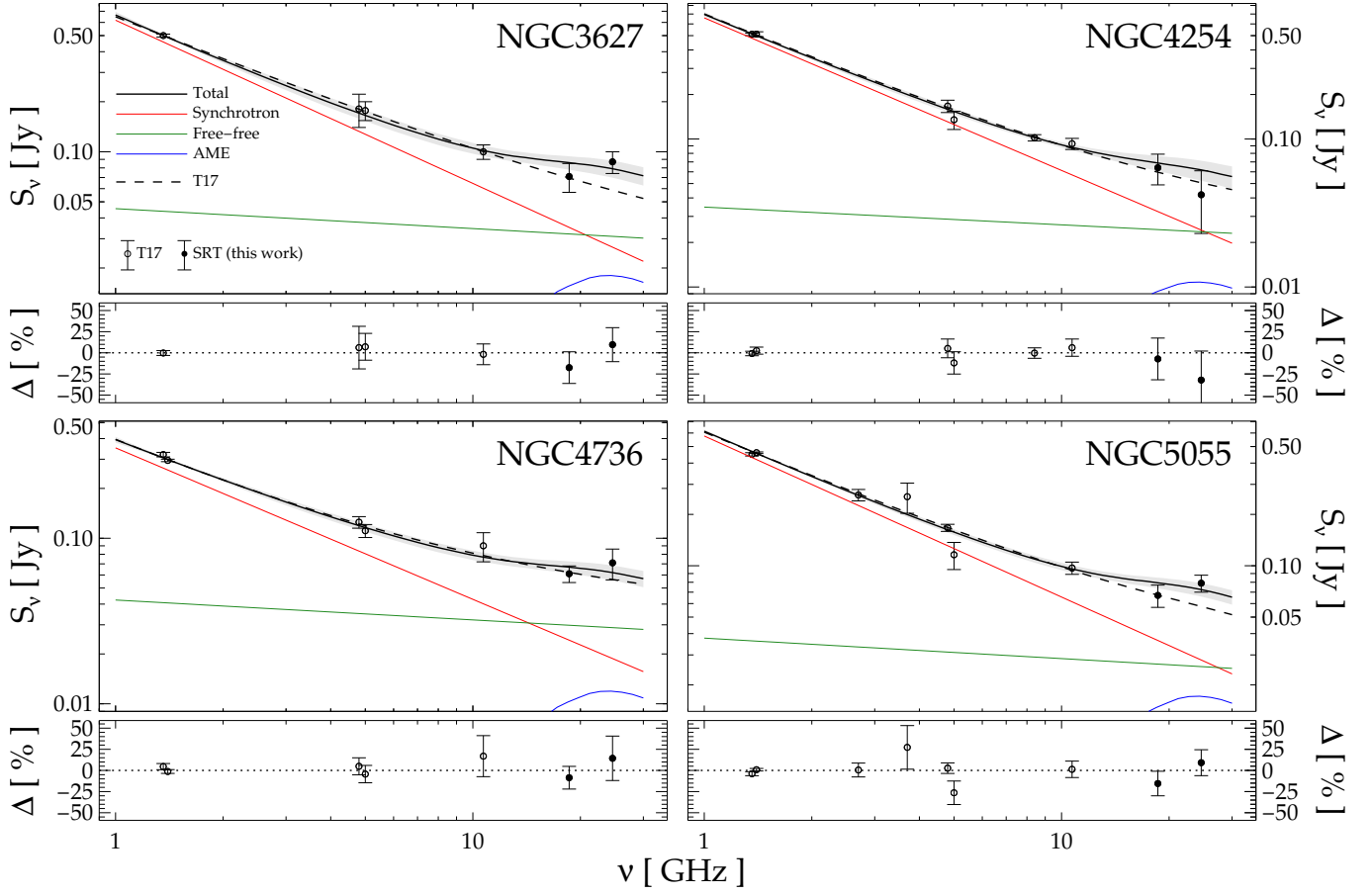
Fig. 2. Global SEDs and fits with their uncertainty. We also show each SED component and the T17 fit. Under each SED, we show the residuals \Delta = \text{data-model} (in percentage of the model).
