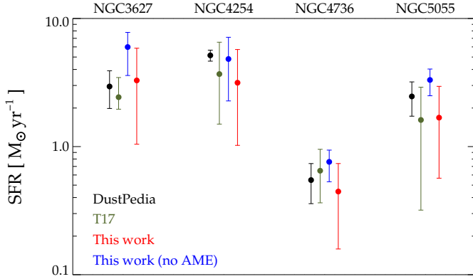
Fig. 3. Comparison between SFRs from DustPedia and from S_{5\text{GHz}}^{\text{ff}} (see text for details).
