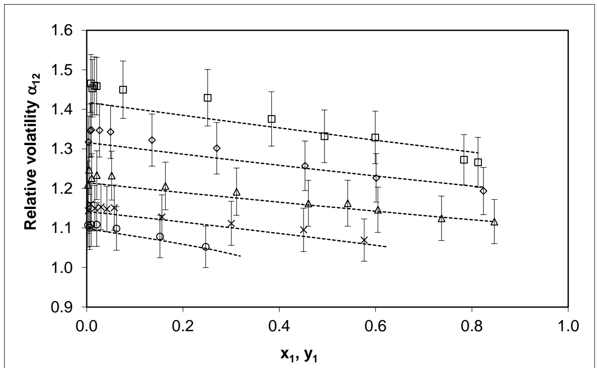
Figure 2a: Variation of the relative volatility \alpha_{12} of the nitrogen (1) + carbon monoxide (2) binary system with liquid composition (whole range of composition) at 100.2 ( \square ), 110.07 ( \diamond ), 120.05 ( \Delta ), 127.07 ( \times ) and 130.07 K ( \circ ) (symbols this work, dashed line: PR EoS). Error bar: 5%.
