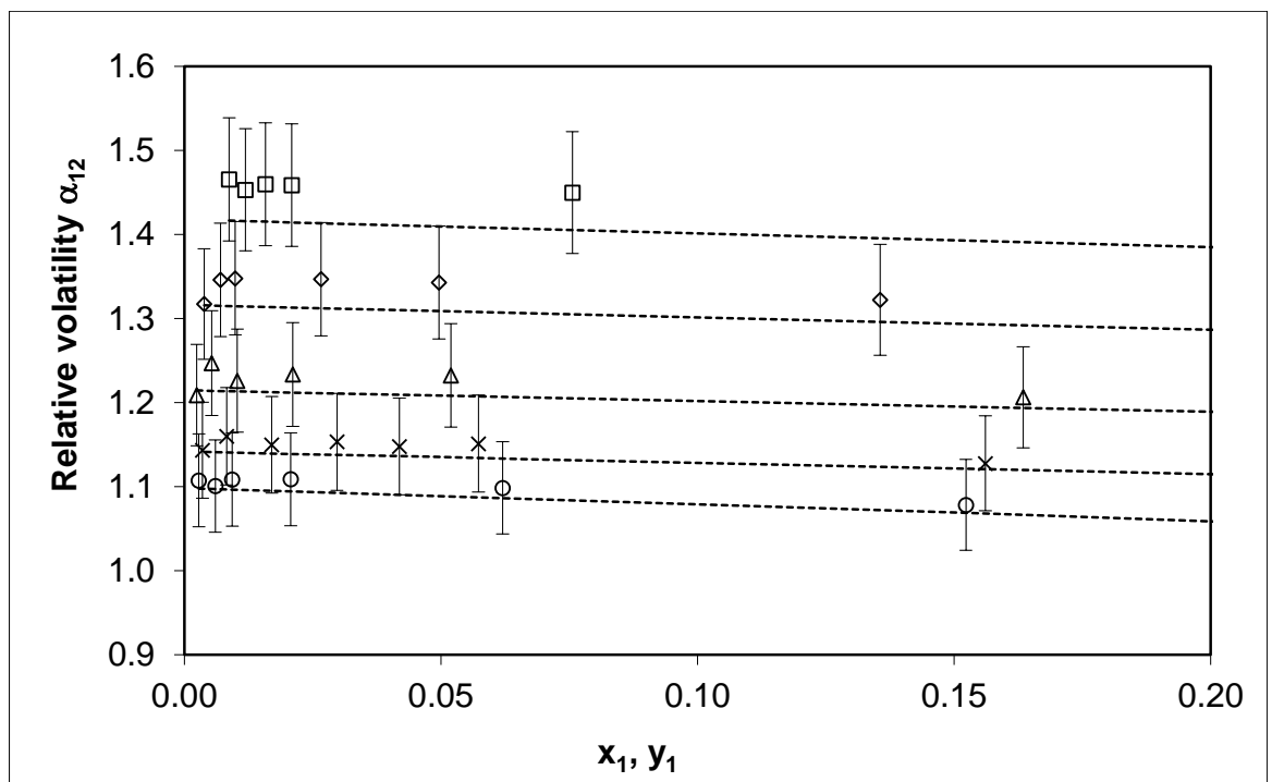
Figure 2b: Variation of the relative volatility \alpha_{12} of the nitrogen (1) + carbon monoxide (2) binary system with liquid composition (between x_1=0 and x_1=0.2 ) at 100.2 ( \square ), 110.07 ( \diamond ), 120.05 ( \Delta ), 127.07 ( \times ) and 130.07 K ( \circ ) (symbols this work, dashed line: PR EoS). Error bar: 5%.
