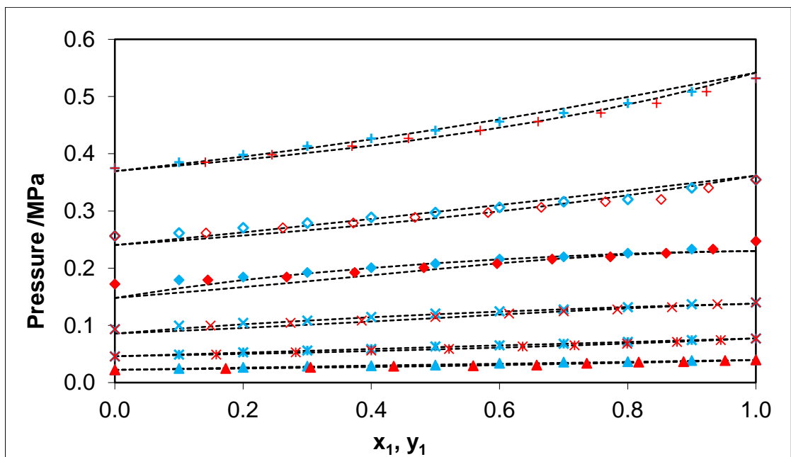
Figure 4b: Vapor liquid Equilibrium data for the nitrogen (1) + carbon monoxide (2) binary system from 70 ( \blacktriangle ), 75 ( * ), 80 ( \times ), 85 ( \blacklozenge ), 90 ( \blacklozenge ) and 95 K ( + ), in blue: bubble point, in red: dew point. Experimental data from Torocheshnikov [8]. Dashed line: Peng Robinson EoS.
