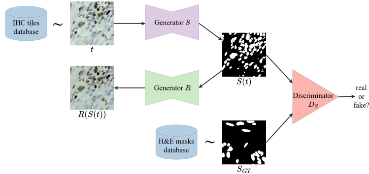
Fig. 1. An overview of our proposed framework. An IHC image t is fed to the generator S , outputting the corresponding segmentation map S(t) . This map is compared to a ground truth mask S_{GT} through discriminator D_S ; and used by the generator R to reproduce the original image R(S(t)) . Similarly, the same process is applied to S_{GT} to generate the corresponding IHC image (not represented here for clarity).
