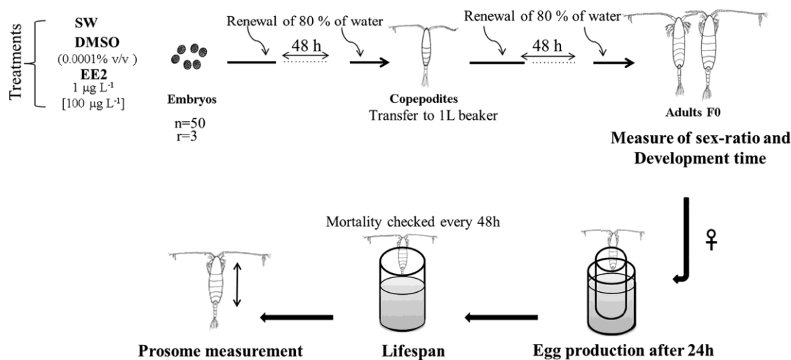
Fig. 1. Experimental setup of (A) acute (48 h) toxicity test using the copepod A. clausi exposed to concentrations of E2 and of EE2 ranging from 0.005 to 5000 \mu g L -1 and (B) chronic toxicity (20 days) test using the copepod A. clausi exposed to concentrations of EE2 of 1 and 100 \mu g L -1 . r = number of replicates; n = number of individuals per replicate; F0: generation 0 of A. clausi ; SW: Sea Water control; DMSO: solvent control containing 0.0001% DMSO (v/v).
