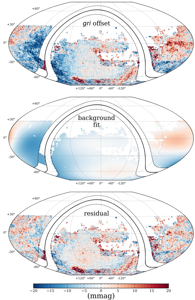
Figure 6. (Top) Offset in the stellar locus (r - i) color at (g - r) = 0.7 fit in each n_{\text{side}}=128 HEALPix pixel relative to the DES value of (r - i)_{\text{DES}} = 0.221 mag. Offsets in this distribution at large spatial scales are likely due to changing stellar populations. (Middle) Polynomial fit to the (r - i) offset map smoothed with a \sigma = 5^{\circ} Gaussian kernel. (Bottom) Map of residuals after the polynomial fit has been subtracted. This residual map highlights variations in the location of the stellar locus at smaller scales and is an estimate of the color uniformity.
