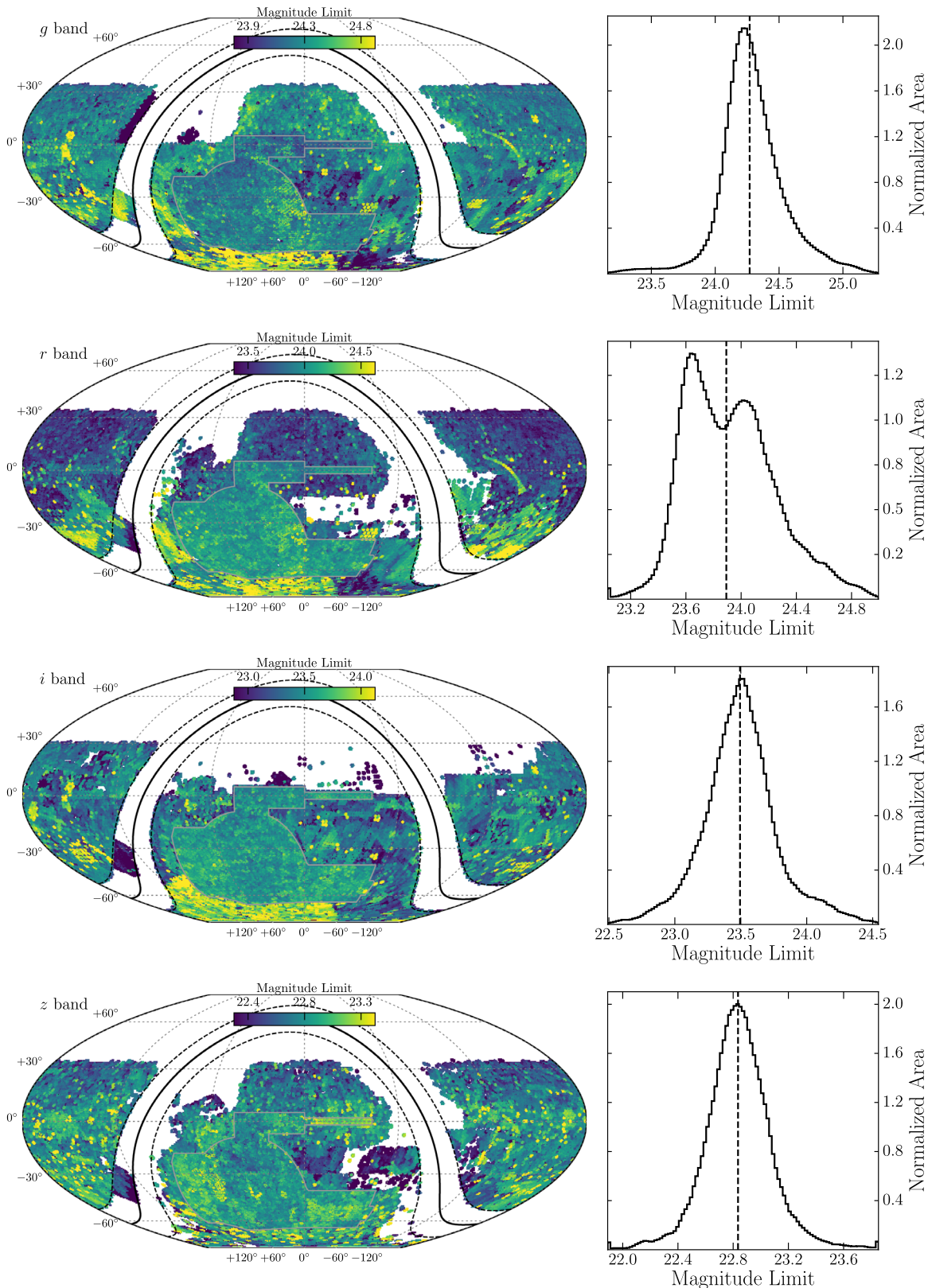
Figure 10. Sky maps and histograms of the S/N = 5 magnitude limit computed from the statistical uncertainty in \text{MAG\_PSF} . Dashed vertical lines indicate the median depth quoted in Table 1. Sky maps are plotted using an equal-area McBryde–Thomas flat polar quartic projection in celestial equatorial coordinates.
