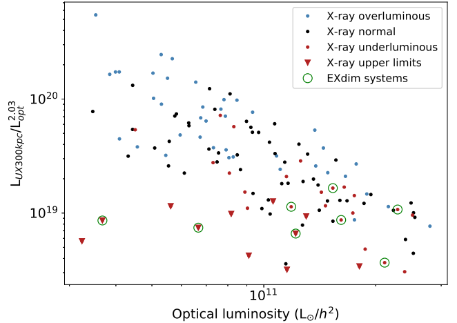
Fig. 16. Ratio of L_{\text{UX300 kpc}}/L_{\text{opt}}^{2.03} ( U_{\text{XO}} ) plotted against L_{\text{opt}} for all groups. Blue, black, and red colours denote groups in the X-ray overluminous, normal, and underluminous subsamples. Inverted triangles denote X-ray upper limits, where no significant X-ray flux value was detected. We highlight X-ray underluminous systems with properties suggesting an evolved group (called here EXdim groups) with green circles. If these groups are dynamically evolved, their low X-ray emission must have some other cause.
