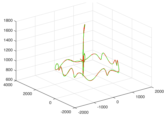
Figure 7. Three-dimensional plot of marker trajectory of the motion of the right wrist (distal; CMU 86 Trial 1). The red curve shows the experimentally observed coordinates and the green curve gives their neural approximations (with two centers and 100 satellites).
