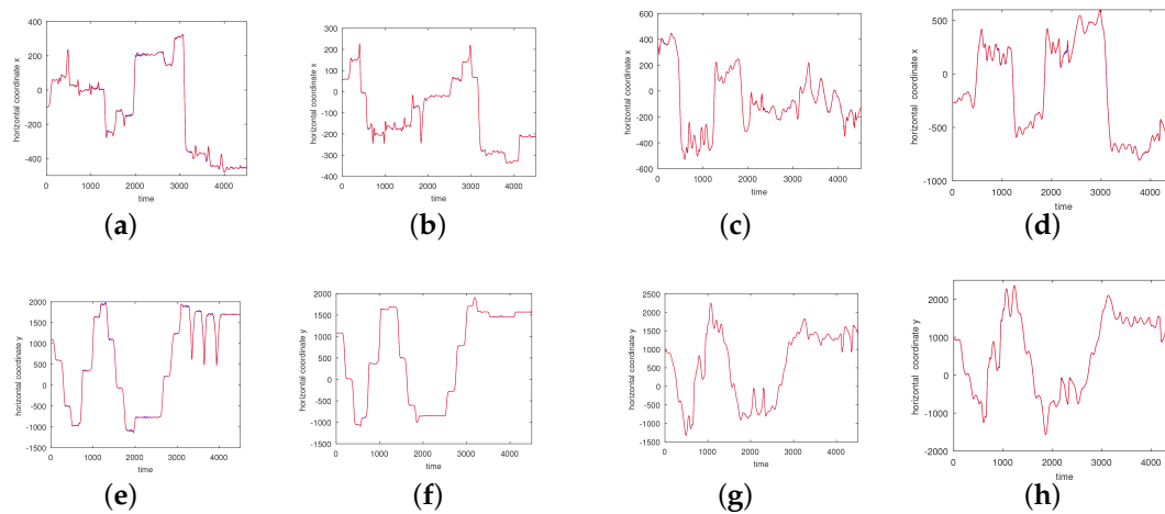
Figure 9. Approximations of x (left) and y coordinates (right) by 200 neurons and two centers for a simple non-segmented motion (sampled at 120 Hz). The center frequencies are 0.30 Hz and 0.72 Hz. (a) Right heel, x -coordinate; (b) Left heel, x -coordinate; (c) Right wrist, distal, x -coordinate; (d) Left wrist, distal, x -coordinate; (e) Right heel, y -coordinate; (f) Left heel, y -coordinate; (g) Right wrist, distal, y -coordinate; (h) Left wrist, distal, y -coordinate. The red curves show the experimentally observed coordinates and the blue curves give their neural approximations. Both curves coincide up to pixel accuracy in many places.
