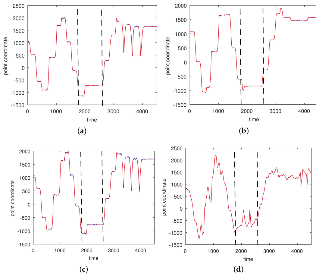
Figure 11. An approximation of y coordinates of a complicated motion (CMU 86 Trial 2; sampled at 120 Hz) by an RBF-network with three centers and 100 satellites. The motion was segmented into three intervals [1, 1800], [1800, 2500], and [2500, 4000]. (a) Right ankle; (b) Left ankle; (c) Right heel; (d) Left wrist, distal. The red curves show the experimentally observed coordinates and the blue curves represent their neural approximations.
