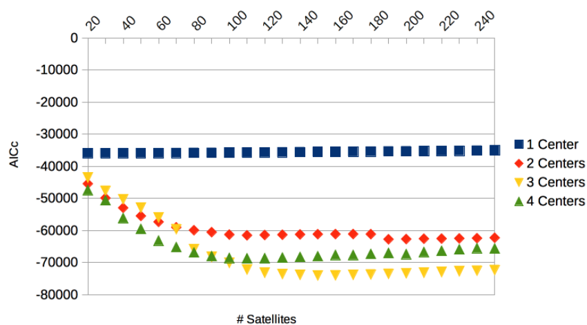
Figure 13. Akaike information criterion corrected for finite sample sizes (AICc) for CMU 86 Trial 1 with 1, 2, 3, and 4 centers and varying numbers of satellites. The global optimum was reached for three centers and 150 satellites.
