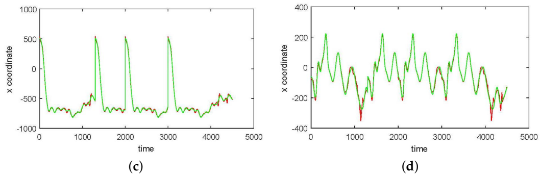
Figure 3. An approximation of x -coordinates by 25 satellites and two centers of motion (CMU 86 Trial 1) consisting of jumping, kicking, and punching (sampled at 120 Hz). (a) Right heel; (b) Left heel; (c) Right wrist, distal; (d) Left wrist, distal. The red curve shows the experimentally observed coordinates and the green curve gives their neural approximations.
