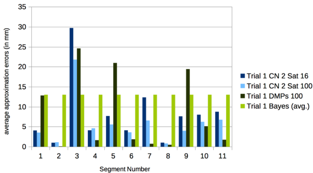
Figure 15. Approximation errors (in mm) for the algorithmically found segments of motions in CMU 86 Trial 1. We give the errors for using 16 and 100 satellites. As a comparison we give the results using rhythmic dynamic movement primitives (DMPs) with 100 basis functions computed with pydmps, and the average approximation error of the Bayesian approach reported in [28] (Table 3). Notice that segments 2, 4, 6, and 8 are short transitional motions between the neighboring segments. The average over all segments is 8.7 mm for the DMPs, 7.9 mm for two centers and 16 satellites, and 6.7 mm for two centers and 100 satellites.
