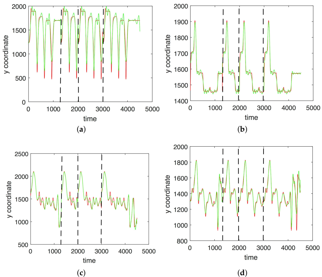
Figure 4. An approximation of y -coordinates by 25 satellites and two centers of motion (CMU 86 Trial 1; sampled at 120 Hz). (a) Right heel; (b) Left heel; (c) Right wrist, distal; (d) Left wrist, distal. The red curve shows the experimentally observed coordinates and the green curve gives their neural approximations.
