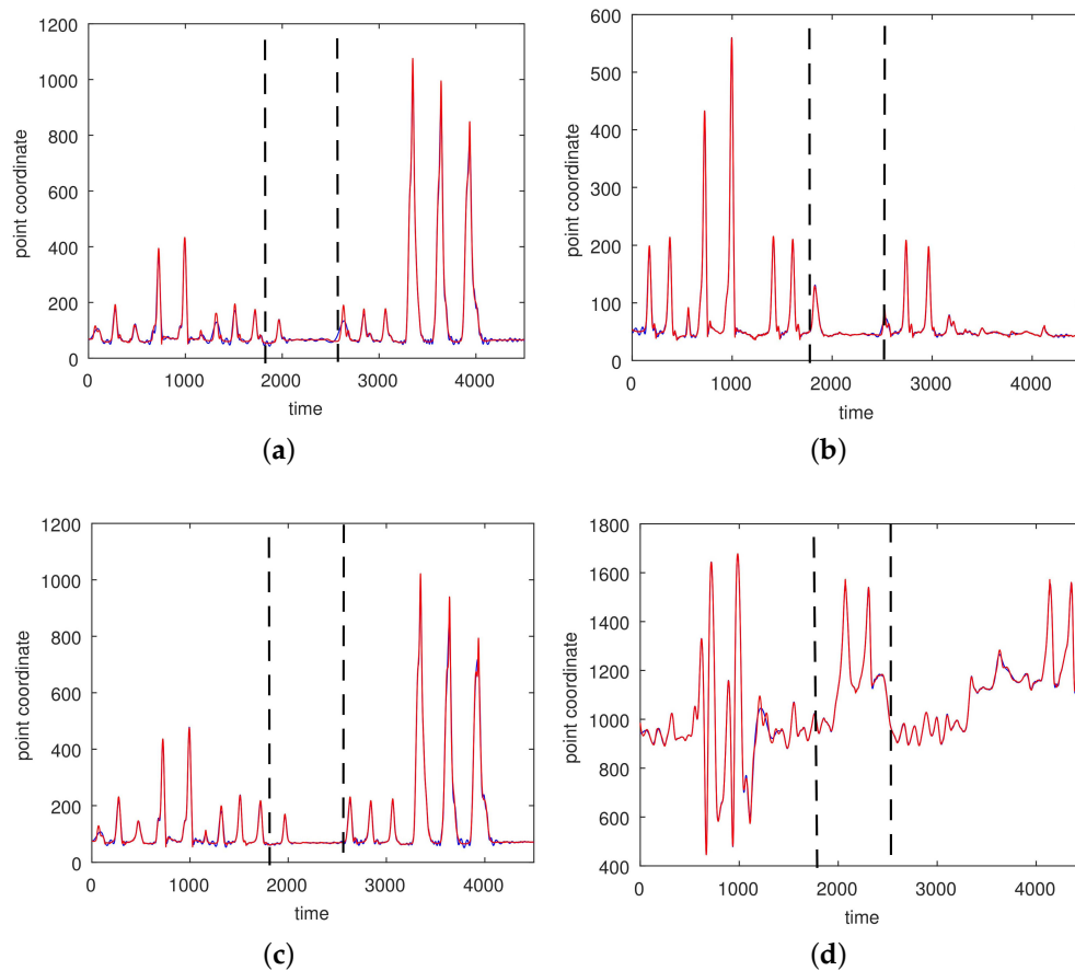
Figure 12. An approximation of the z coordinates of a complicated motion (CMU 86 Trial 2; sampled at 120 Hz) by an RBF-network with three centers and 100 satellites. The motion was segmented into three intervals [1, 1800], [1800, 2500], and [2500, 4000]. (a) Right ankle; (b) Left ankle; (c) Right heel; (d) Left wrist, distal. The red curves show the experimentally observed coordinates and the blue curves represent their neural approximations.
