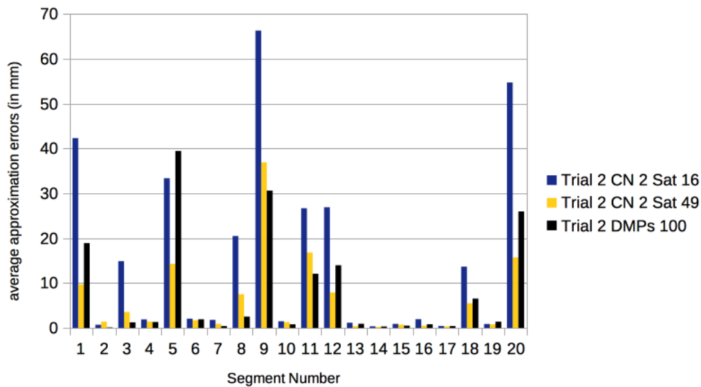
Figure 16. Approximation errors (in mm) for the algorithmically found segments of motions in CMU 86 Trial 2. We give the errors for using 16 satellites and 49 satellites. As a comparison we give the results using rhythmic DMPs with 100 basis functions computed with pydmps. The average over all segments is 8.0 mm for the DMPs, 15.6 mm for two centers and 16 satellites, and 6.3 mm for two centers and 49 satellites.
