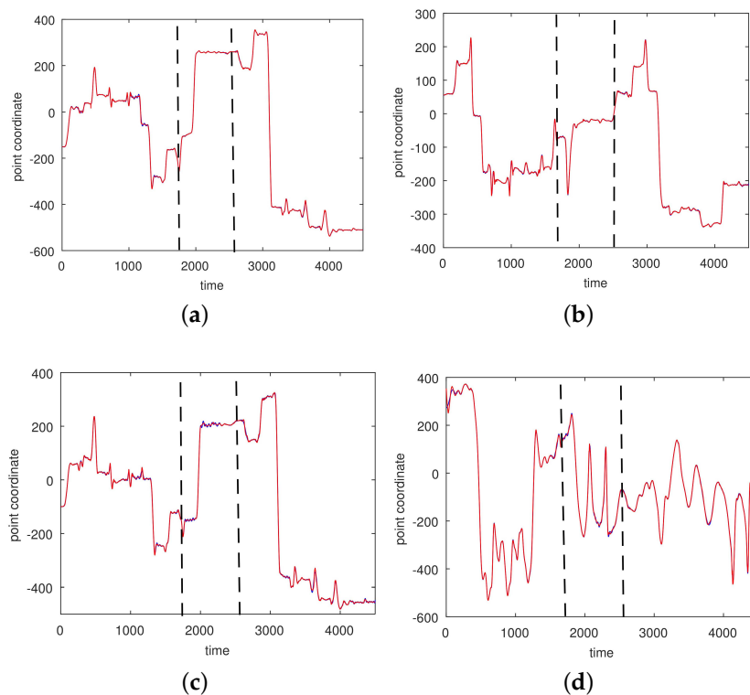
Figure 10. Approximations of x coordinates of a complicated motion (CMU 86 Trial 2; sampled at 120 Hz) by a radial basis function (RBF) network with three centers and 100 satellites. The motion was segmented into three intervals [1, 1800], [1800, 2500], and [2500, 4000]. (a) Right heel; (b) Left heel; (c) Right wrist, distal; (d) Left wrist, distal.
