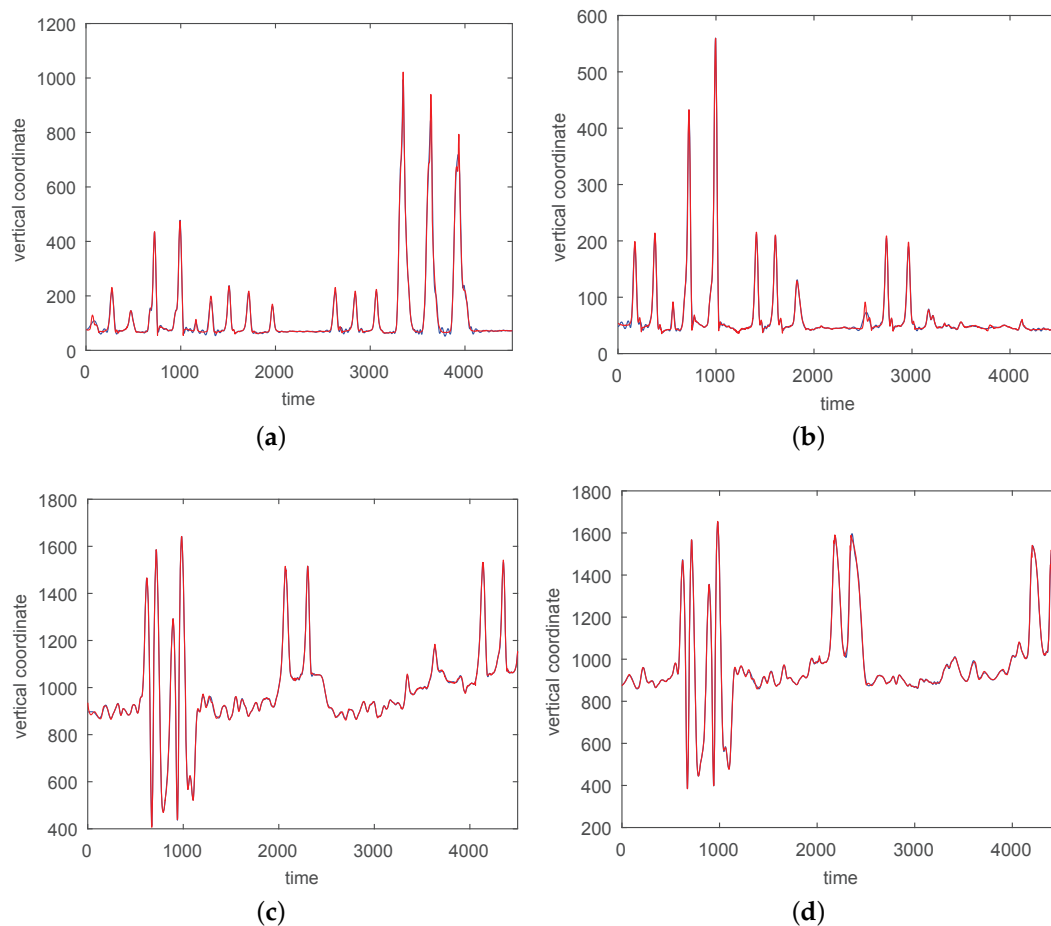
Figure 8. An approximation of z (vertical) coordinates by 200 neurons and two centers for a simple non-segmented motion (sampled at 120 Hz). The center frequencies are 0.30 Hz and 0.72 Hz. (a) z -coordinate for the right heel; (b) The left heel; (c) z -coordinate for the right wrist, distal; (d) The left wrist, distal. The red curves show the experimentally observed coordinates and the blue curves give their neural approximations.
