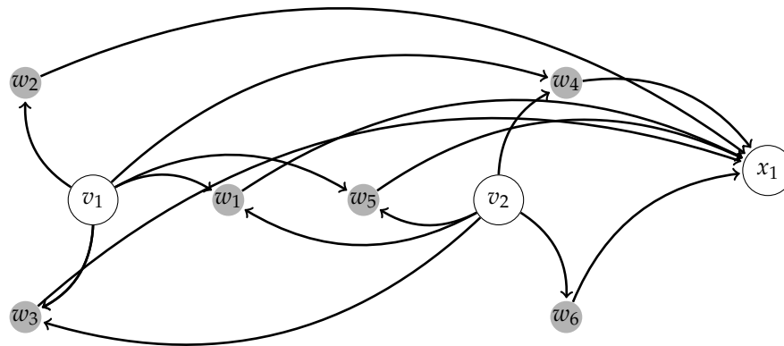
Figure 1. This image shows the control of one of the x -coordinates of human body motions by a network consisting of two oscillators ( v_1, v_2 ) and a radial basis function (RBF) network with N = 6 nodes. The graph consists of eight nodes denoted by v_1, v_2, w_1, w_2, w_3, w_4, w_5, w_6 . Each node w_i corresponds to a contribution of a radial basis function \Phi(q - \bar{q}^{(i)}) . The nodes v_1, v_2 form the set of centers \mathcal{C} and they affect w_i . In turn, the nodes w_i determine the output coordinate x_1 .
