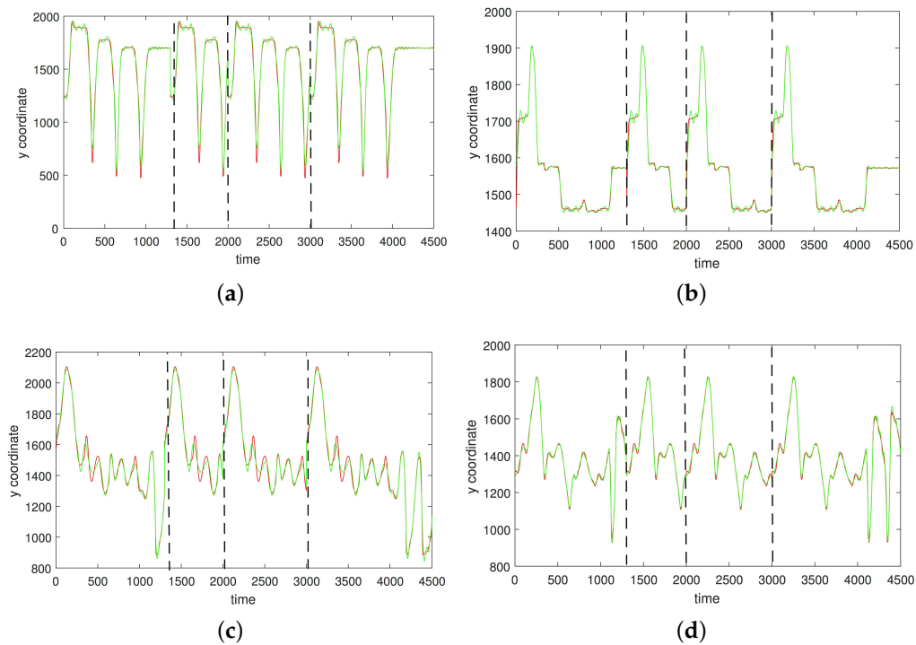
Figure 5. An approximation of y -coordinates by 50 satellites and two centers of motion (CMU 86 Trial 1; sampled at 120 Hz). (a) Right heel; (b) Left heel; (c) Right wrist, distal; (d) Left wrist, distal. The red curve shows the experimentally observed coordinates and the green curve gives their neural approximations.
