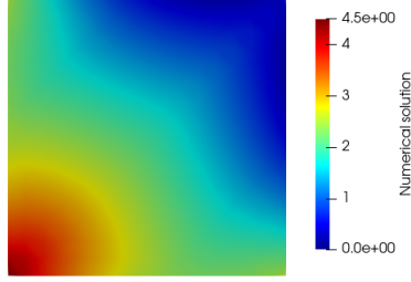
Fig. 4 Test 2: numerical solution on the third mesh.
