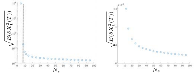
Fig. 4: Impact of sensor number N_s on the noise of X(T) , i.e the square root of the variance of \delta X(T) for fixed \sigma_N = 10^{-2} , T_0 = 80s , T = 100s , T_e = 120s , f = 100Hz and N = 100 . (a) shows the sharp transition nearby N_s = 8 in semi-log representation. (b) Same data as in (a) but in normal plot within N_s range between 10 to 95.
