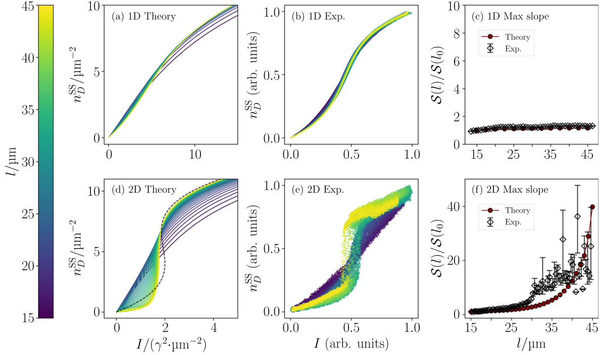
FIG. 2. (a) [(b)] Theoretical (experimental) results for the steady-state polariton density n_D^{SS} averaged over the probing disk as a function of the drive intensity I for different top-hat spot sizes l (see color bar) in the 1D configuration with detuning \Delta = \gamma . (c) The maximum derivative S(l) for each top-hat size l normalized by the maximum derivative at l_0 = 15 \mu\text{m} , for both theoretical and experimental results (see legend). (d)–(f) The same quantities as in (a)–(c) for the 2D configuration. The dashed line in (d) is the prediction of the mean-field theory in Eq. (5). Note that as the top hat increases in size, the slope in the 1D configuration quickly saturates for increasing size l , while in the 2D configuration the slope sharply increases in both theory and experiment, as expected for a first order phase transition.
