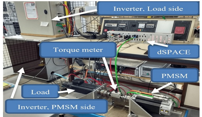
Fig. 4. Test bench
