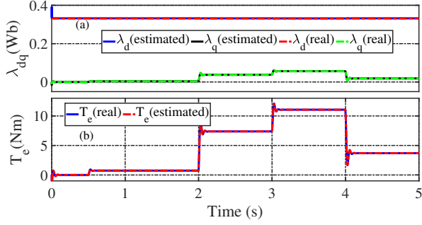
Fig. 2. Simulation results: (a) real and estimated flux linkages, (b) real and estimated electromagnetic torque
