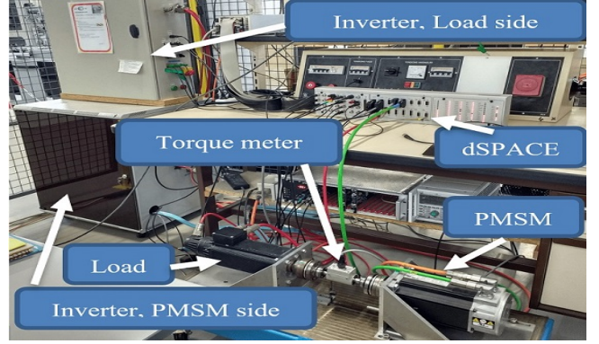
Fig. 4. Test bench
