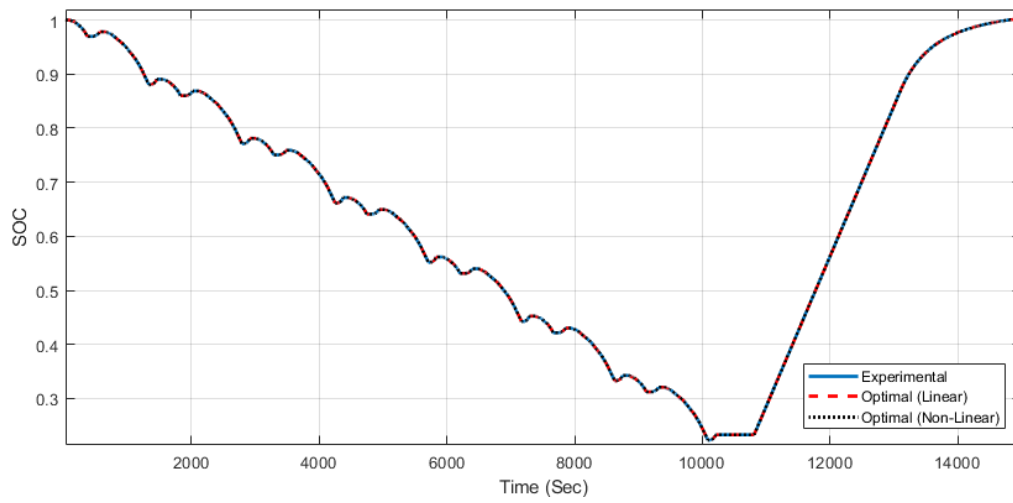
Figure 15: State of charge experimental and modeling responses
