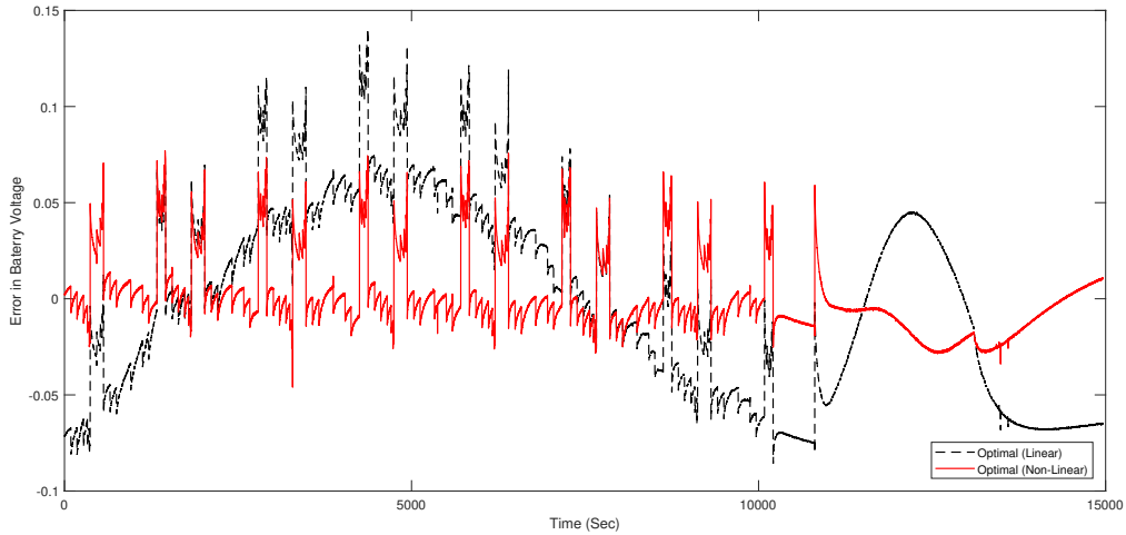
Figure 13: Error response of the battery voltage
