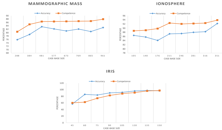
Fig. 6: Comparing estimated competence using our CEC-Model to the CB's accuracy for Mammographic Mass, Ionosphere, and Iris data sets
