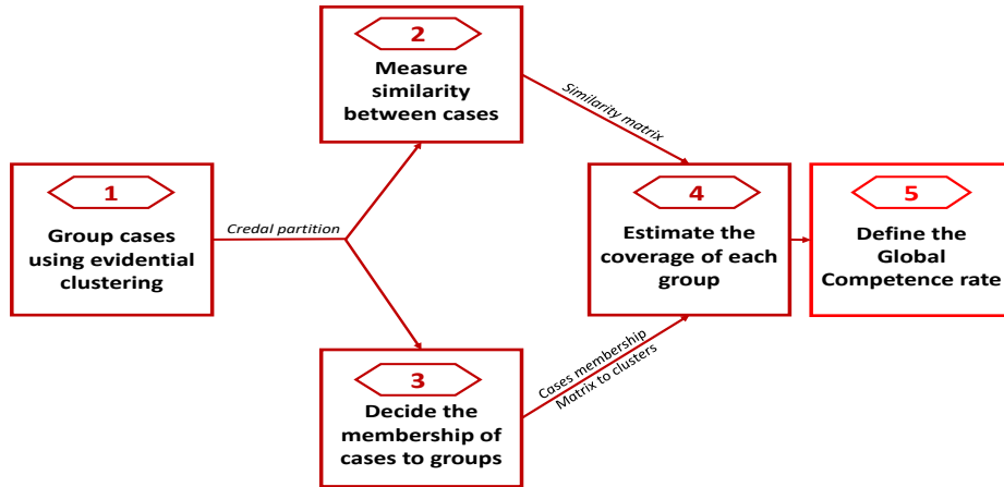
Fig. 5: CEC-Model steps for CB's competence estimation
