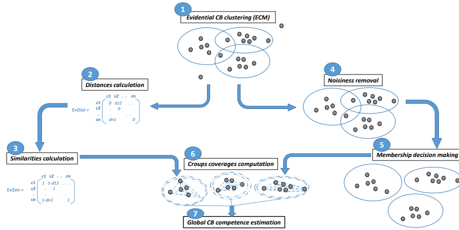
Fig. 1. CEC-Model's process
