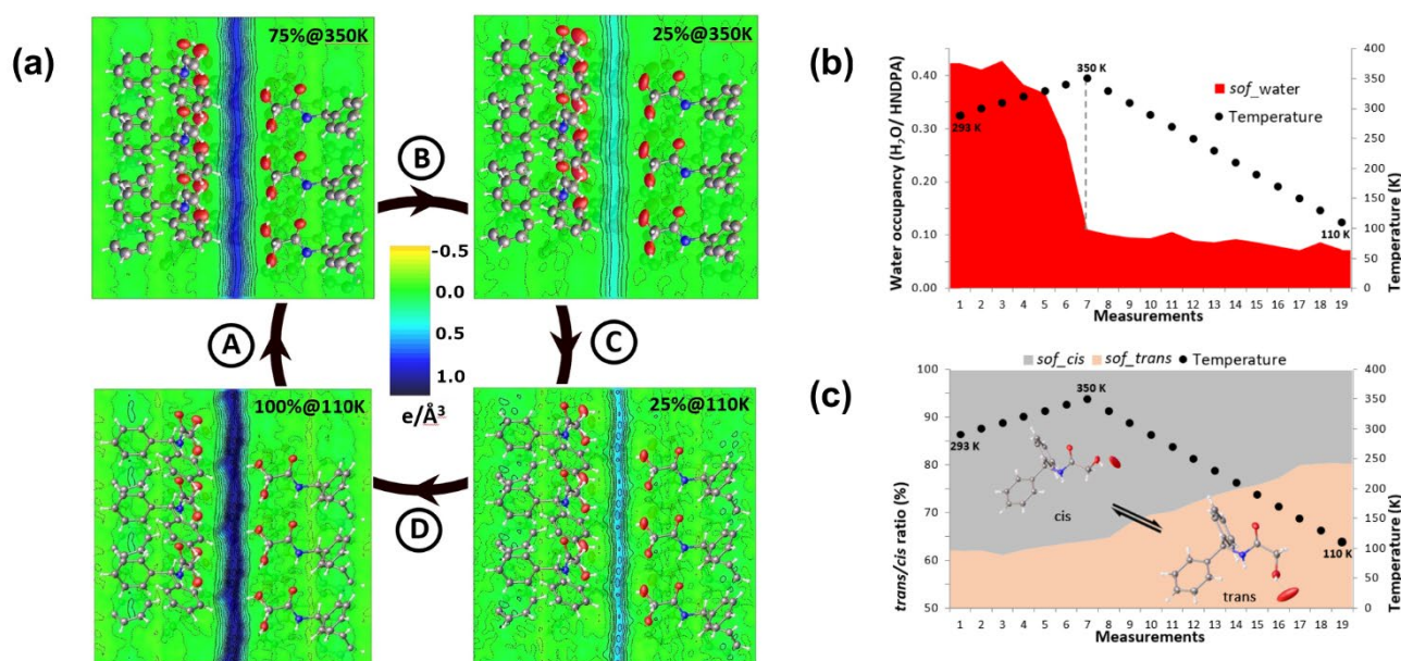
Figure 3. Water release-reuptake cycle and water flow inside the water channel as a function of temperature. (a) The figures represent electron density in a lengthwise cross-section of the water channel (front HNDPA molecules have been removed for clarity) with the experimental electron density shown as a color scale ( e/\text{\AA}^3 ); the dark blue color represents the highest electron density values. The water occupancy is expressed in percentage (%) considering that 0.4 was the maximum possible occupancy. A. Temperature increase from 100 to 350 K. B. Sample left at 350 K for 1 h. C. Temperature decrease at 100 K. D. Sample left at 293 K in air for 24 h and diffraction experiment at 100 K. (b-c) Focus on the water release event (from 293 up to 350 K and back to 100 K, 60 min interval). (b) Channel water occupancy and (c) cis/trans conformation (%), plotted as a function of temperature, expressed by the measurement number. Site occupancy factor (sof) e.s.d.'s are all in the range of 0.005.
