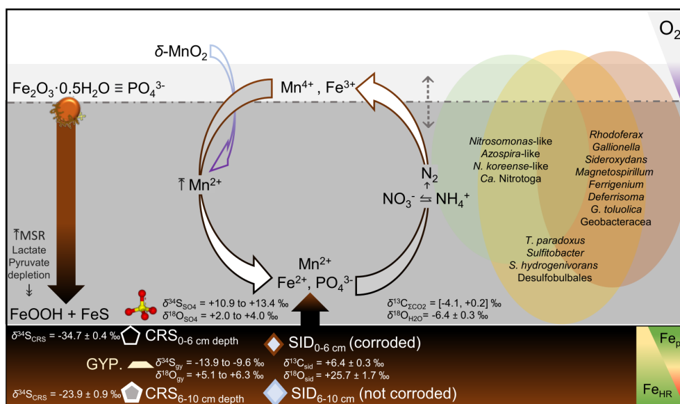
Figure 7. Scheme summarizing the speciation and stable isotopes ranges of sulfur-bearing phases (pyrite, \text{S}^0 : CRS; gypsum: GYP; siderite: SID) and the biogeochemical cycling mechanisms likely operating in the redox-stratified Lake Medard and its SWI. (Background colours as in Fig. 2.) The prokaryote groups depicted represent nitrate-, iron- and sulfur-utilizing species identified via 16S rRNA gene amplicon sequencing (see text for details).
