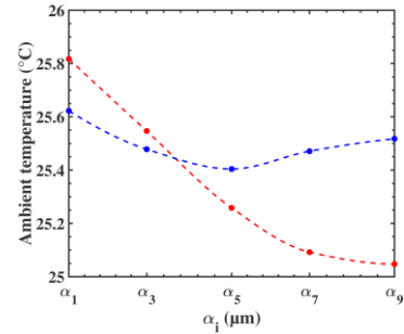
Figure 4. Evolution of the required ambient temperature to achieve 34^\circ\text{C} as a function of geometrical parameters for a skin covered with a non-structured (blue) and structured (red) membrane.
