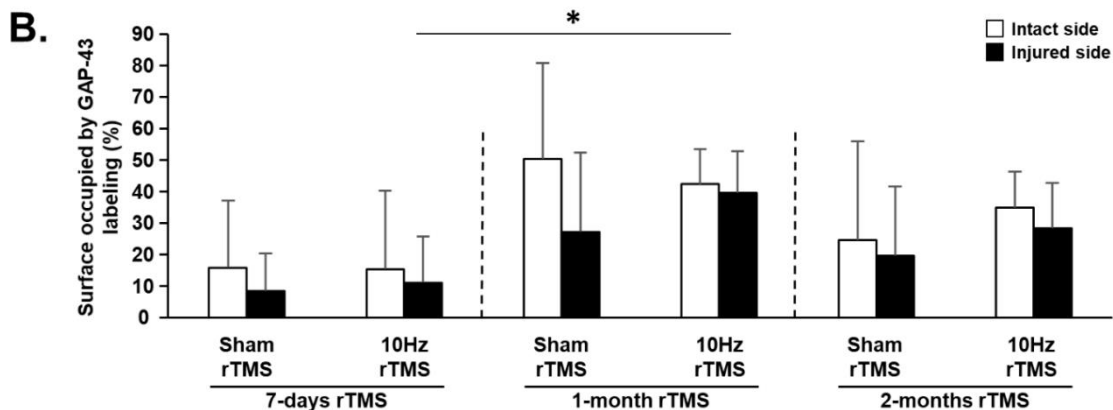
Figure 7. GAP-43 expression approximate to phrenic motoneurons following C2 hemisection: (A) representative images showing the surface occupied by GAP-43 labeling around denervated phrenic motoneurons labeled with CTB in C2 hemisected rats, following 7 days, 1 month, or 2 months of Sham or 10 Hz rTMS treatment; (B) quantification of the area occupied by GAP-43 labeling approximate to phrenic motoneurons on the intact and injured sides of Sham or 10 Hz rTMS-treated C2 hemisected animals following 7 days, 1 month, or 2 months of treatment. There is no difference between the intact and the injured sides for the different groups (paired t -test for intact vs. injured side, p > 0.05 ; * 7-day 10 Hz rTMS compared with 1-month 10 Hz rTMS for the injured side (Student's t -test, p = 0.017 ).
