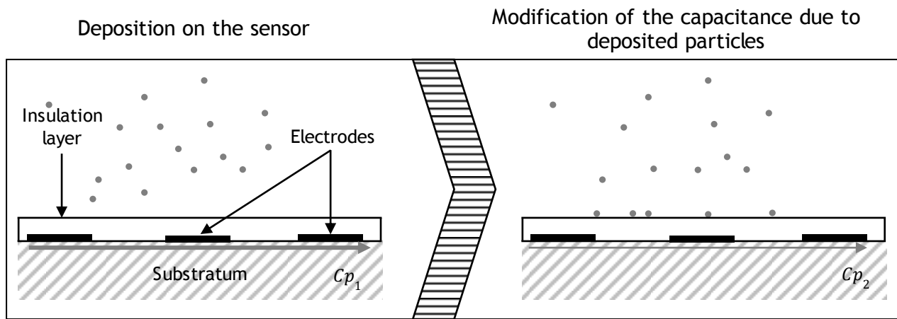
Figure 8: Operation of a capacitive sensor
