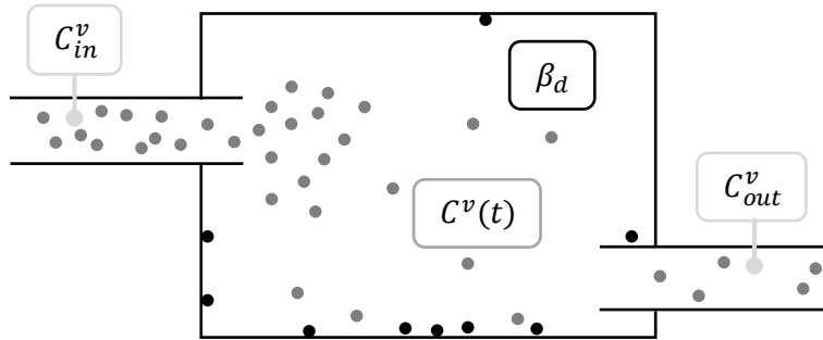
Figure 2: Global deposition in a room with flux conservation
