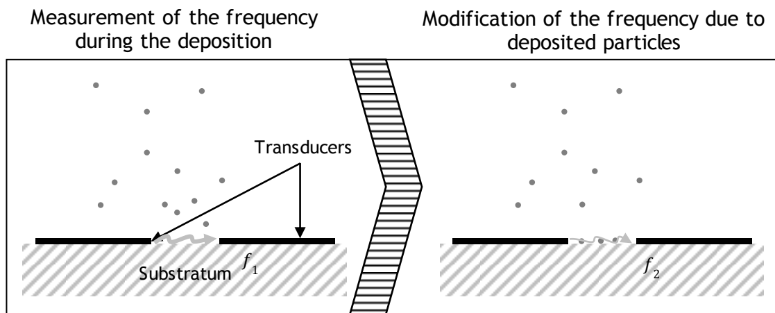
Figure 4: Operation of a Surface Acoustic Wave (SAW) sensor
