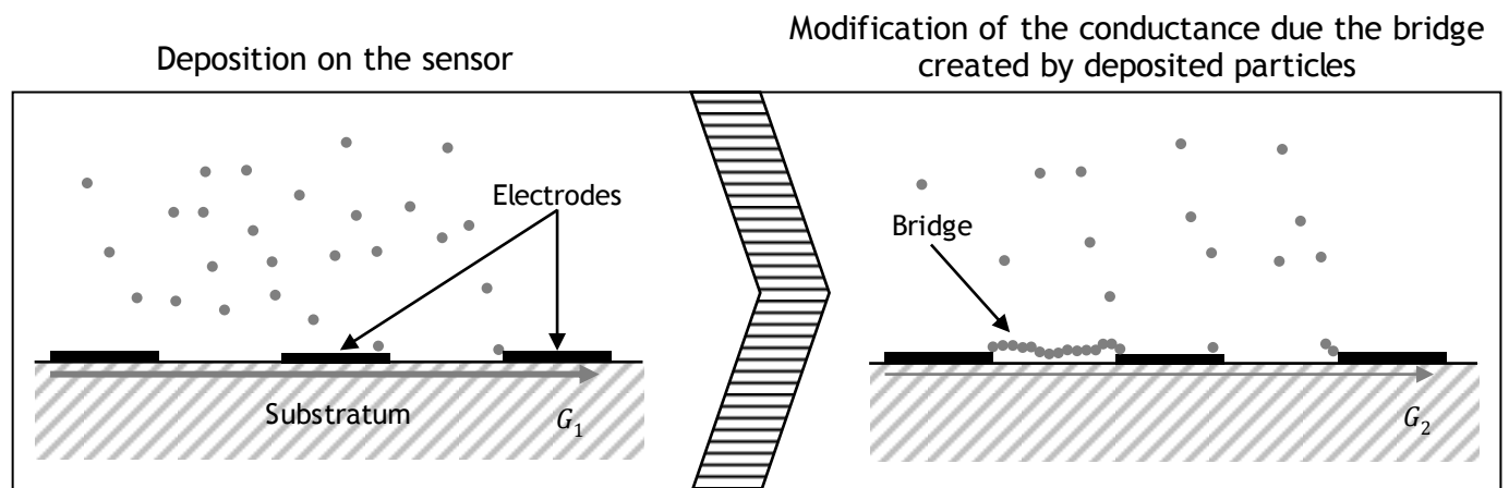
Figure 7: Operation of a resistive sensor
