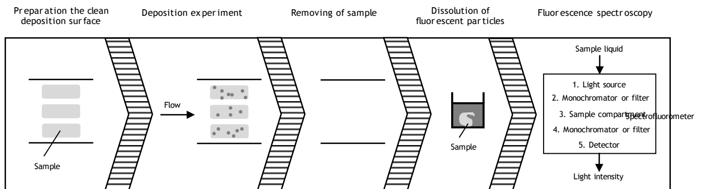
Figure 3: Fluorescence spectroscopy – stages
