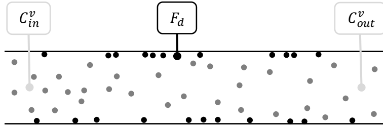
Figure 1: Global deposition in a channel with flux conservation
