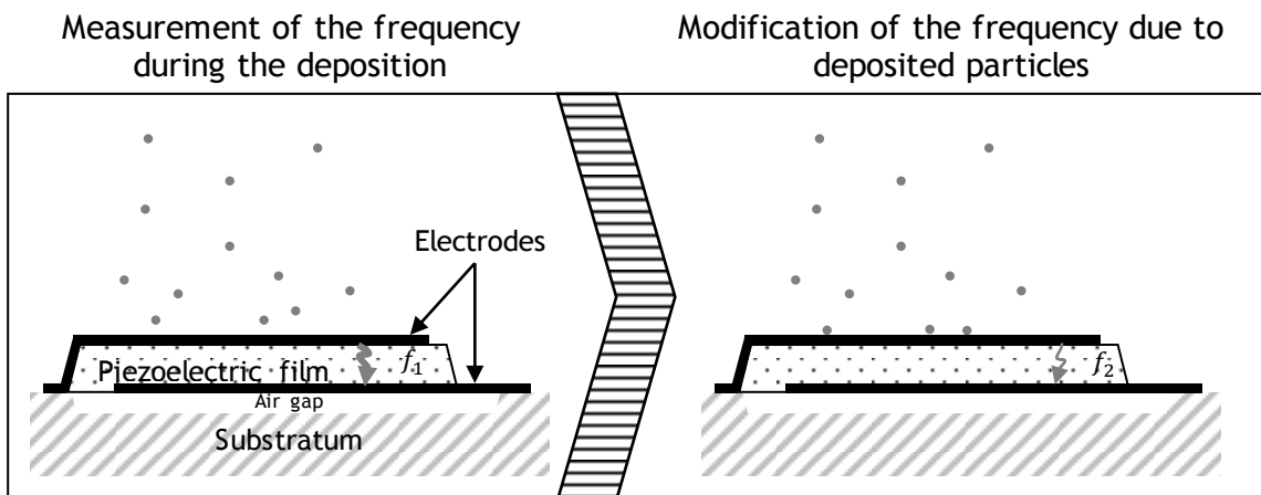
Figure 5: Operation of a Film Bulk Acoustic Resonator (FBAR)
