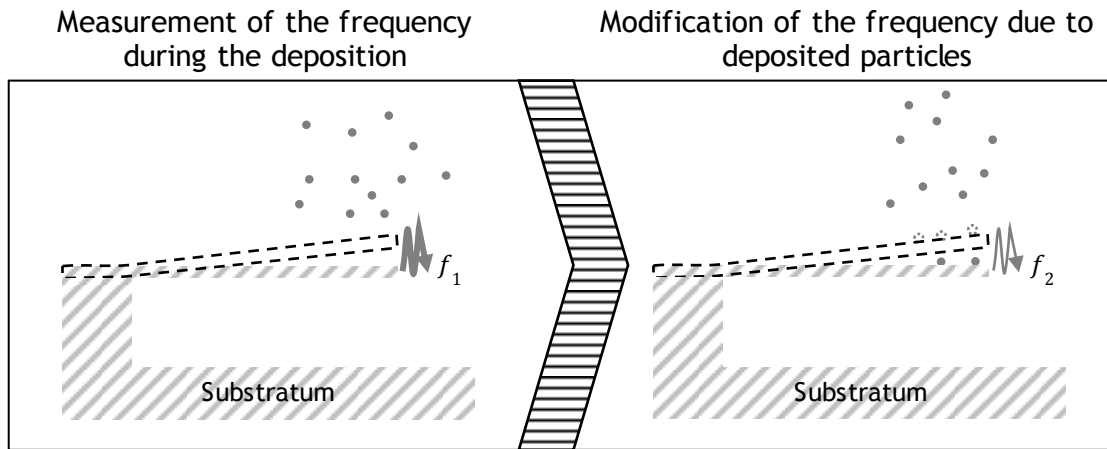
Figure 6: Operation of a cantilever Micro-Electro-Mechanical System (MEMS)
