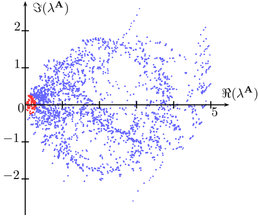
FIGURE 2. Real and complex parts, resp. \Re(\lambda^{\mathbf{A}}) and \Im(\lambda^{\mathbf{A}}) , of the spectrum \lambda^{\mathbf{A}} of matrix \mathbf{A} for \mathcal{D}_\Omega = 6 .
