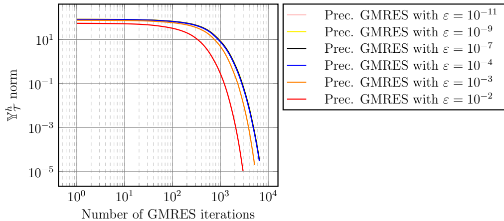
FIGURE 6. Comparison of the convergence rate of the preconditioned GMRES UWVF with basis reduction for different values of the threshold \varepsilon .
