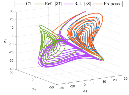
(a) Phase portrait
