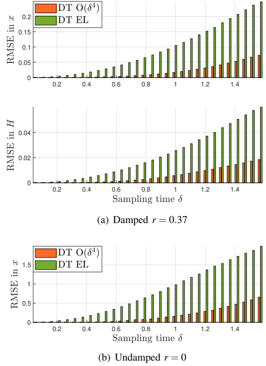
Fig. 1. Pendulum: RMSE in the state x and Hamiltonian H at the sampling instants \delta \in [0, \frac{\pi}{2}] with x_0 = \text{col}\{\frac{\pi}{2}, 0\} .
