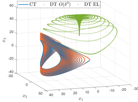
(a) Phase portrait
