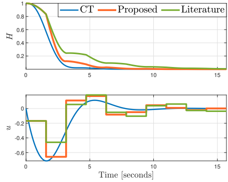
(b) Hamiltonian and control effort
