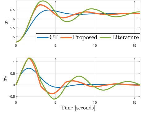
(a) State trajectories
