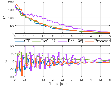
(b) Control effort and Hamiltonian evolution
