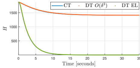
(b) Hamiltonian evolution
