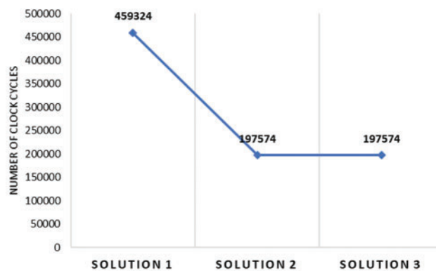
Figure 8: Comparison of the number of clock cycles for HLS solutions
