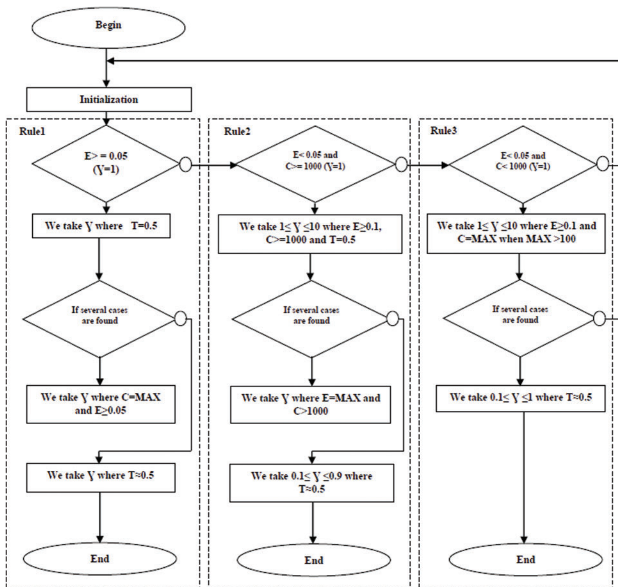
Figure 3: The GCM rules
