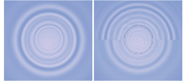
Figure 10: Left: a full levelset simulation of one drop in the water in a deep pool. Right: a levelset simulation (in the center ring) coupled with 2D wave propagation using shallow water dispersion (top) and deep water dispersion (bottom). The dispersion law used by the 2D simulator has a significant effect on the resulting wave pattern and coupling, and should be chosen to match the 3D simulation.
