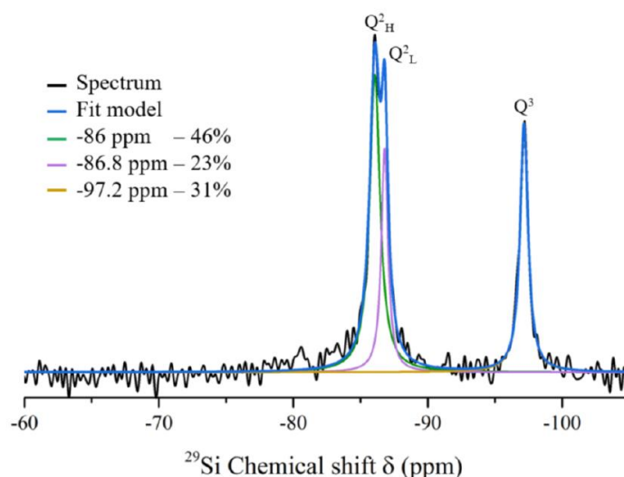
Fig. 8. ^{29}\text{Si} MAS NMR spectrum of xonotlite synthesized under supercritical conditions at 25 MPa and 400 °C in 7 s.
