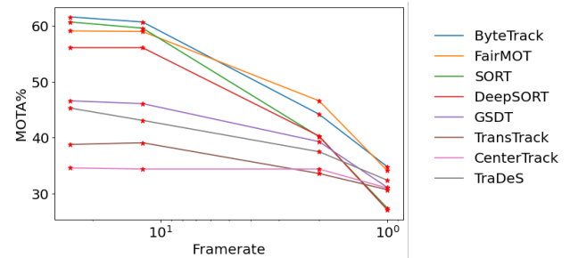
Figure 1: Multi object tracking accuracy (metric MOTA [11]) of different tracking methods on the MOT20-01 sequence [2] with different framerates (logarithmic scale). As the framerate is reduced, and thus the change between frames increases, all methods suffer a significant drop in performance.
