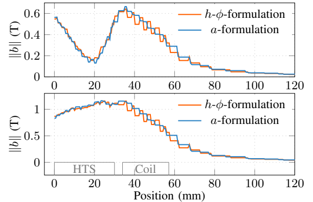
Fig. 3: Norm of the magnetic flux density at \varepsilon = 2 \text{ mm} above the system, along the dashed line represented in Fig. 1. The upper plot is at t = 0.25 T and the lower plot at t = 3.5 T . Curves from h -, h - \phi - a -, h - \phi - b -formulations are indistinguishable from that of the h -formulation ( h -conform field in air). The same is true for curves from \bar{a} -, h - a -, a - j -formulations in comparison with those from the a -formulation ( b -conform field in air).
