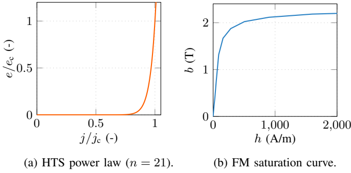
Fig. 2: Nonlinear laws involved in the problem.
